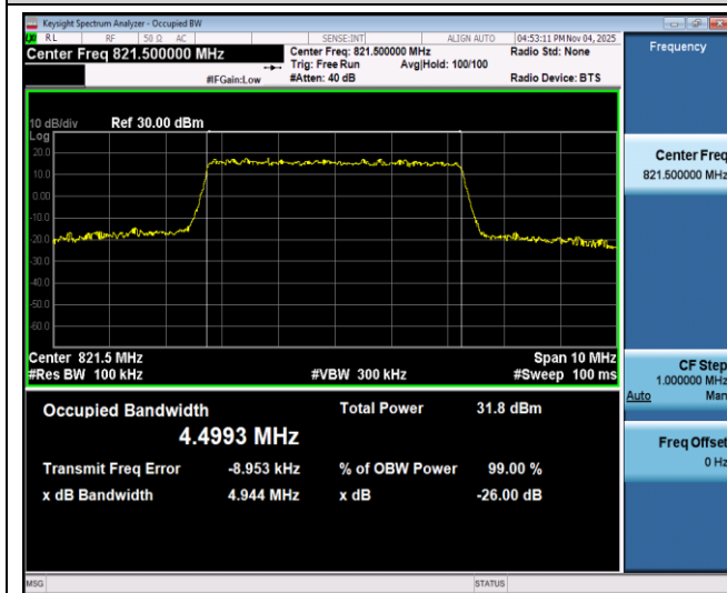
Band26-5MHz-QPSK-26915-25RB#0
