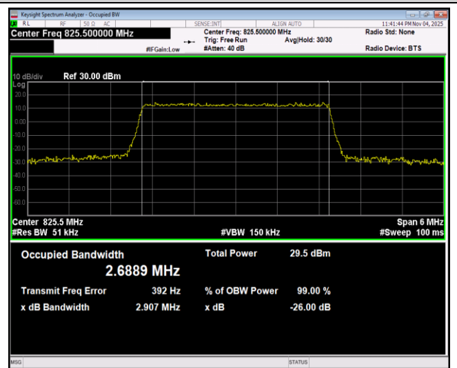
Band26-3MHz-64QAM-27025-15RB#0
