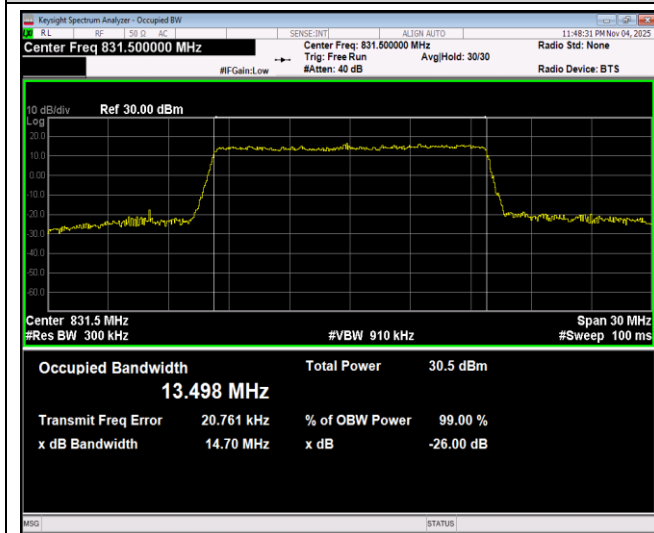
Band26-15MHz-64QAM-26965-75RB#0
