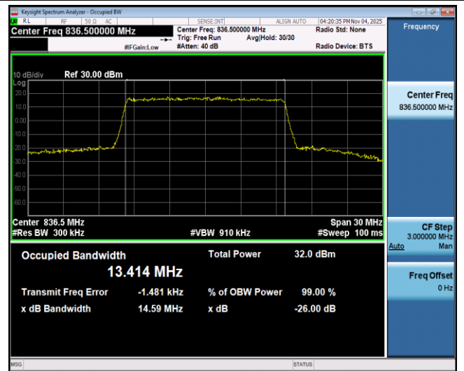
Band26-15MHz-QPSK-26915-75RB#0
