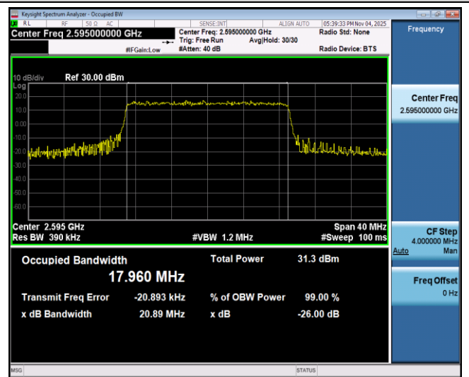
Band38-20MHz-16QAM-37850-100RB#0
