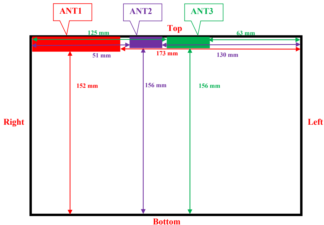
EUT Back View
