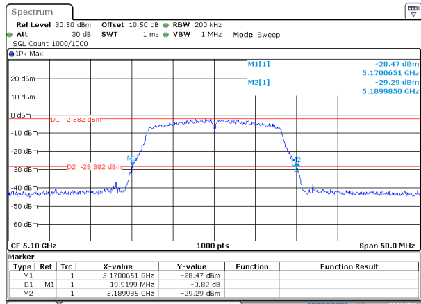
802.11a_5180MHz
