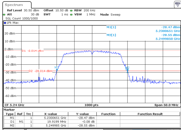
802.11a_5240MHz
