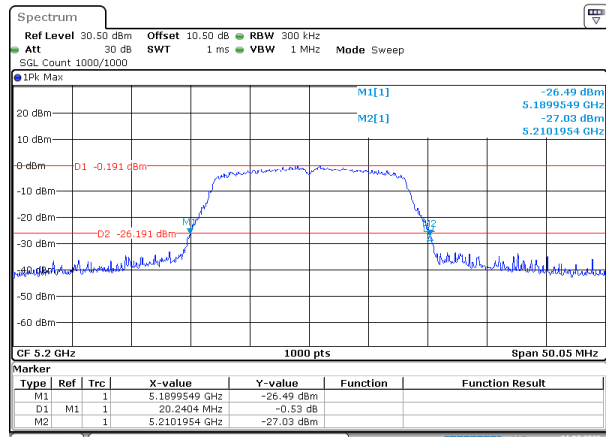
802.11a_5200MHz
