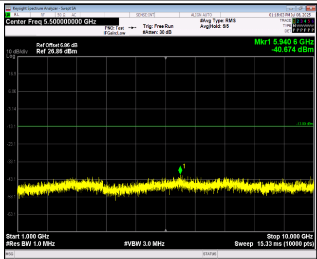
Band5-10MHz-64QAM-20450-1RB#0-Range2:1000~10000MHz
