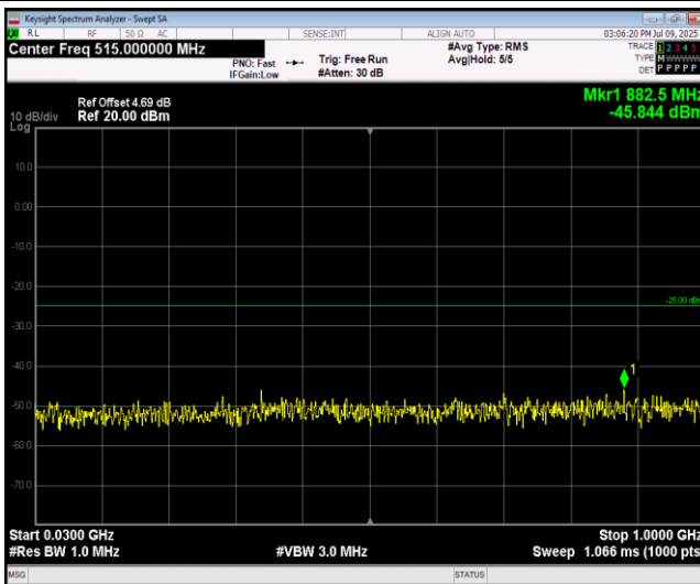
Band7-20MHz-64QAM-21350-1RB#0-Range1:30~1000MHz
