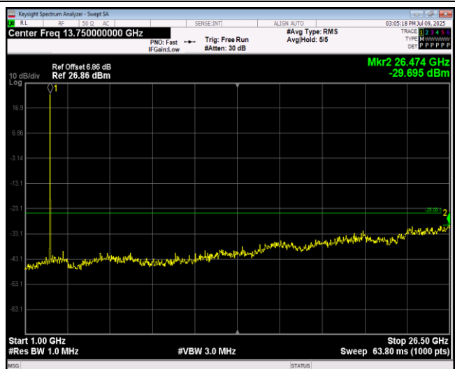
Band7-20MHz-16QAM-21100-1RB#0-Range2:1000~ 26500MHz
