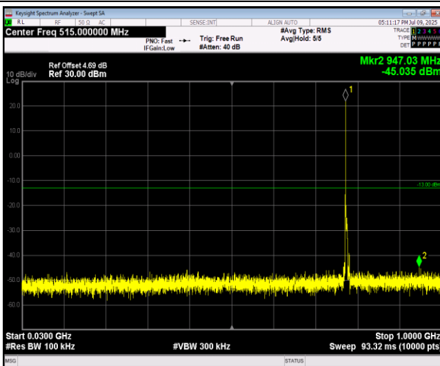
Band13-5MHz-64QAM-23230-1RB#0-Range1:30~1000MHz
