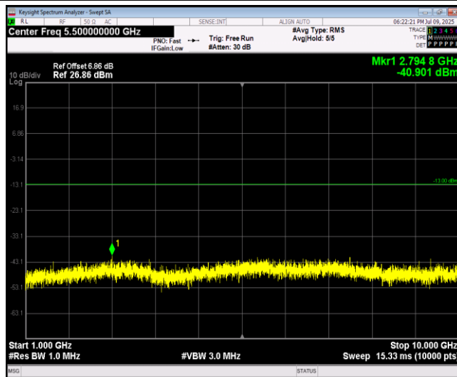
Band17-5MHz-16QAM-23790-1RB#0-Range2:1000~10000MHz
