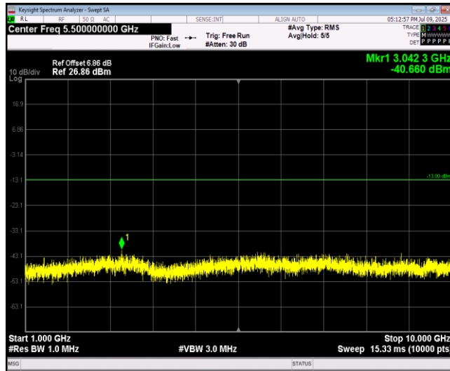
Band13-5MHz-64QAM-23205-1RB#0-Range2:1000~10000MHz
