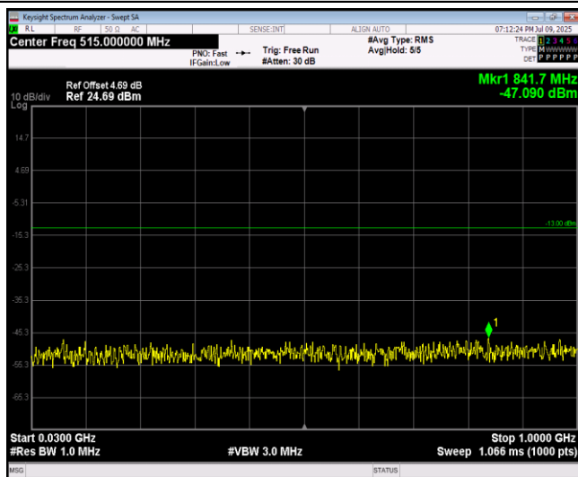
Band25-1.4MHz-64QAM-26365-1RB#0-Range1:30~1 000MHz
