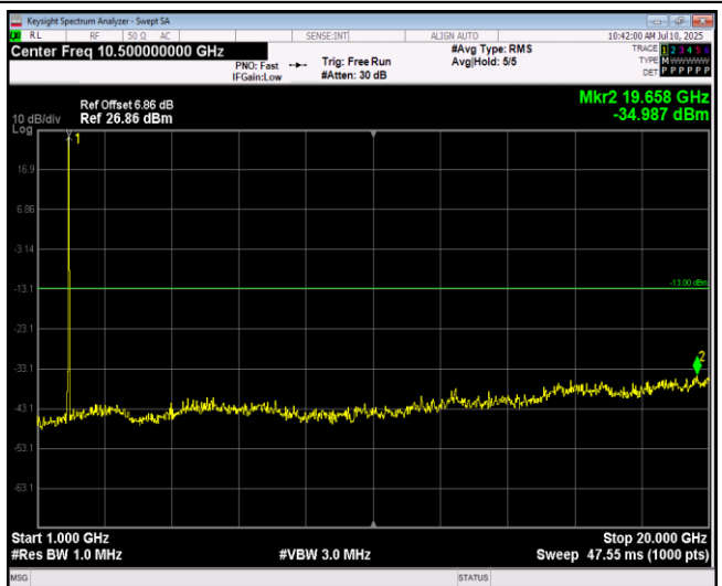
Band25-20MHz-16QAM-26140-1RB#0-Range2:1000~20000MHz
