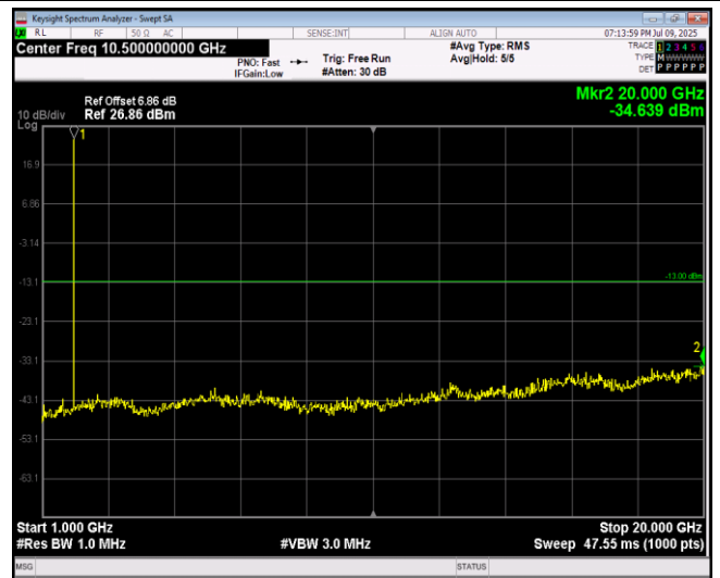
Band25-1.4MHz-64QAM-26047-1RB#0-Range2:1000 ~20000MHz
