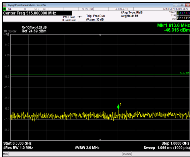
Band25-1.4MHz-64QAM-26047-1RB#0-Range1:30~1 000MHz
