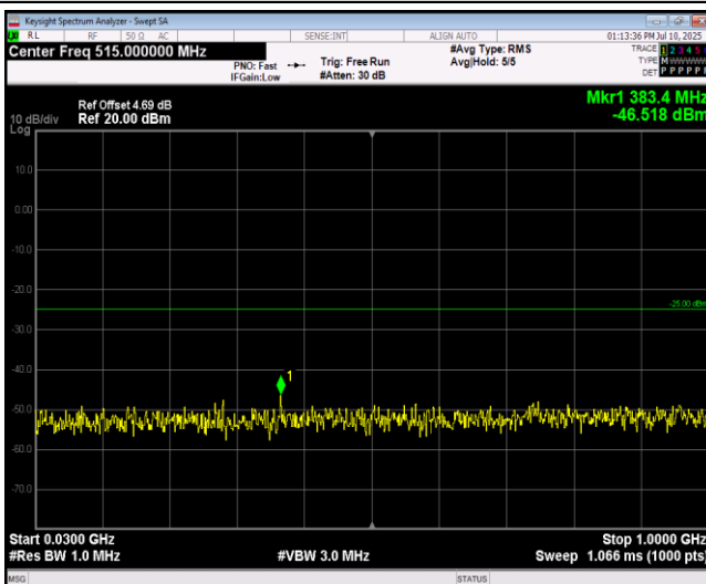
Band38-20MHz-QPSK-37850-1RB#0-Range1:30~1000MHz
