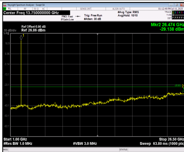
Band38-5MHz-64QAM-38225-1RB#0-Range2:1000~26500MHz
