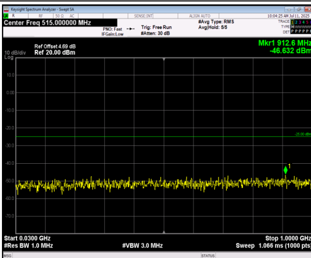
Band41-5MHz-64QAM-40065-1RB#0-Range1:30~1000MHz
