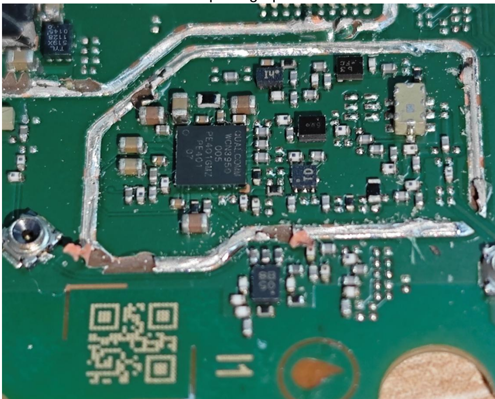
Internal photograph of EUT
