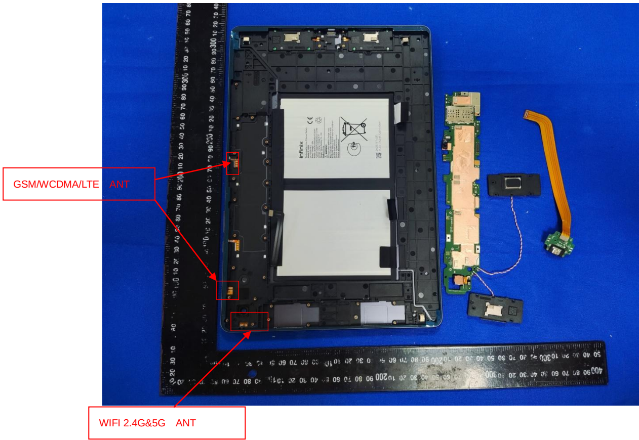
Internal photograph of EUT
