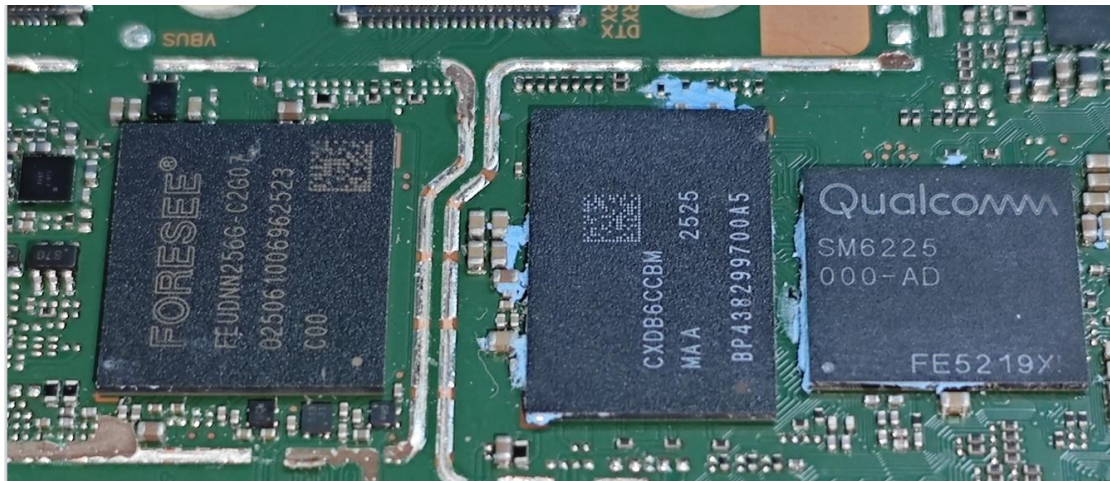
Internal photograph of EUT
