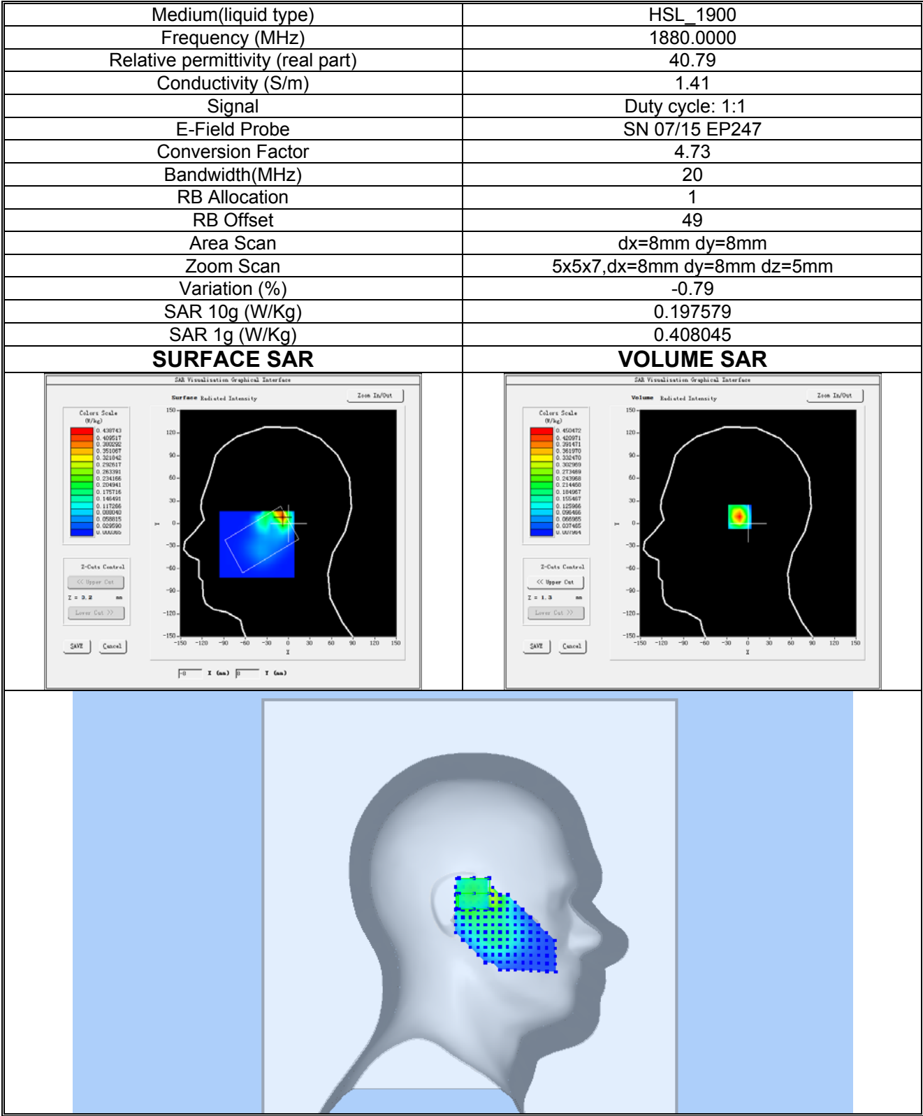
Plot 11:LTE BAND2, Middle channel (Left Head Cheek) Product Description:Mobile Phone Test Date: 2019-10-18
