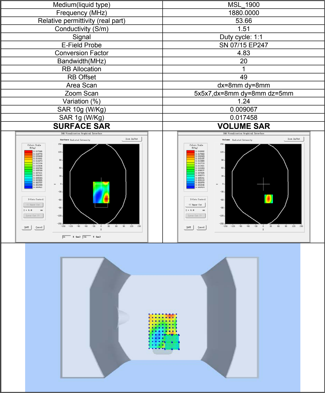
Plot 12:LTE BAND2, Middle channel (Body-worn/Hotspot, Back Surface) Product Description:Mobile Phone Test Date: 2019-10-18
