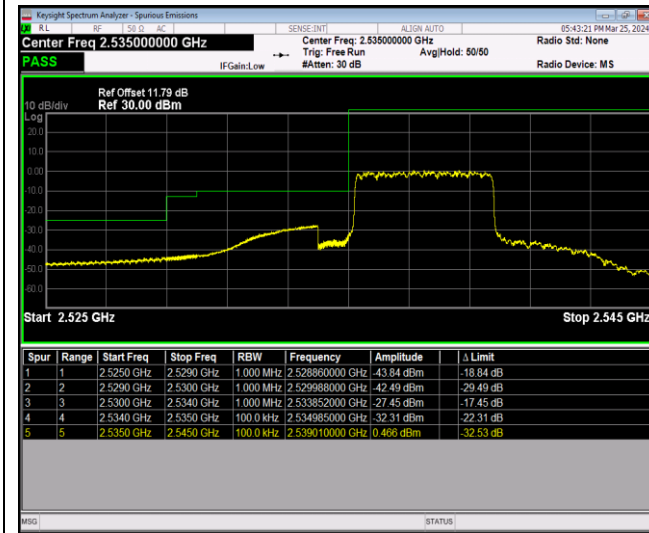
Band41-5MHz-16QAM-41215-1RB#24
