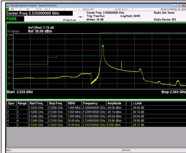
Band41-5MHz-16QAM-40065-25RB#0
