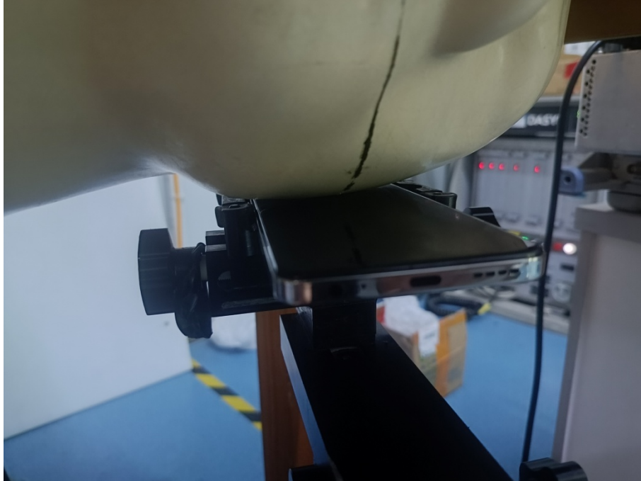
Head Left Cheek Setup Photo (0mm)
