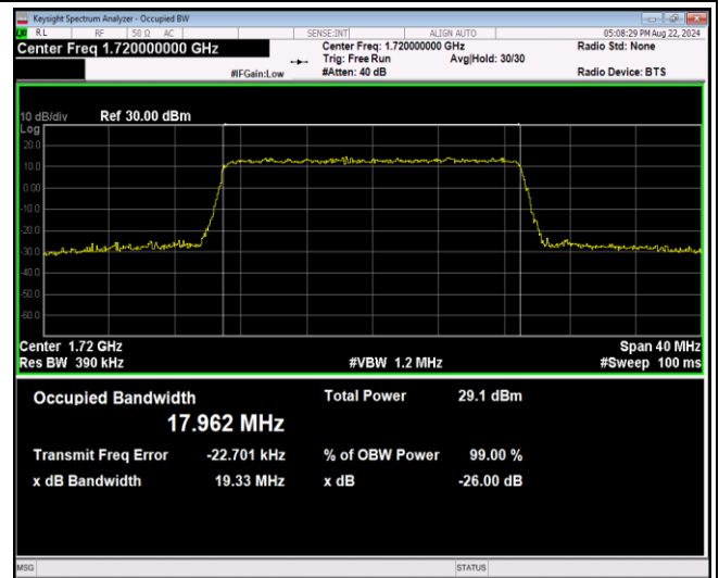
Band4-20MHz-64QAM-20300-100RB#0
