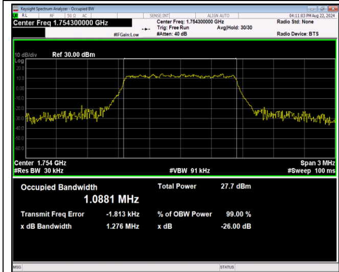
Band4-3MHz-QPSK-20175-15RB#0
