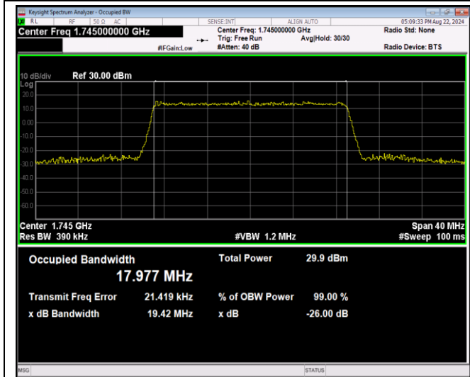
Band4-20MHz-64QAM-20175-100RB#0
