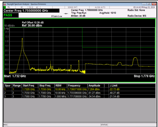
Band4-20MHz-64QAM-20300-100RB#0
