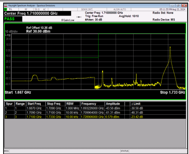
Band4-20MHz-64QAM-20300-1RB#0
