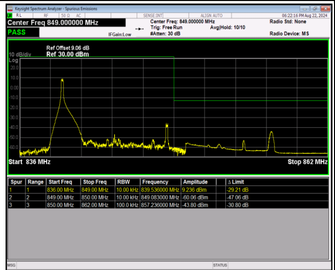
Band5-10MHz-64QAM-20600-50RB#0
