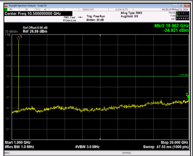
Band4-1.4MHz-64QAM-19957-1RB#0-Range2:1000~20000MHz
