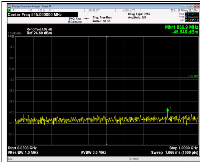
Band2-1.4MHz-64QAM-19193-1RB#0-Range1:30~1000MHz
