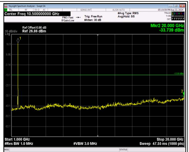
Band4-20MHz-64QAM-20050-1RB#0-Range2:1000~ 20000MHz
