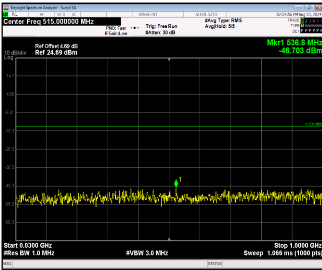
Band2-1.4MHz-QPSK-18900-1RB#0-Range1:30~100 0MHz
