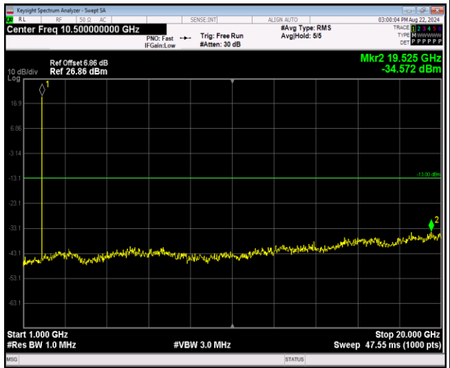
Band2-1.4MHz-QPSK-18900-1RB#0-Range2:1000~ 20000MHz
