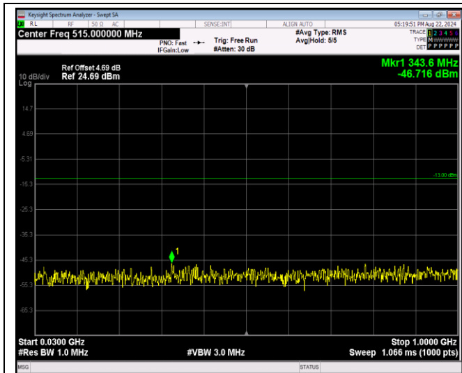
Band4-20MHz-64QAM-20050-1RB#0-Range1:30~100 OMHz
