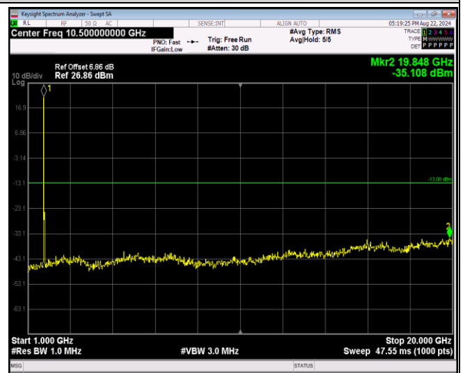
Band4-20MHz-64QAM-20175-1RB#0-Range2:1000~ 20000MHz
