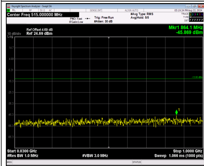
Band4-20MHz-QPSK-20300-1RB#0-Range1:30~1000 MHz
