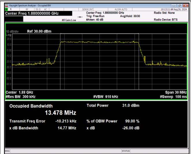
Band2-15MHz-16QAM-18675-75RB#0
