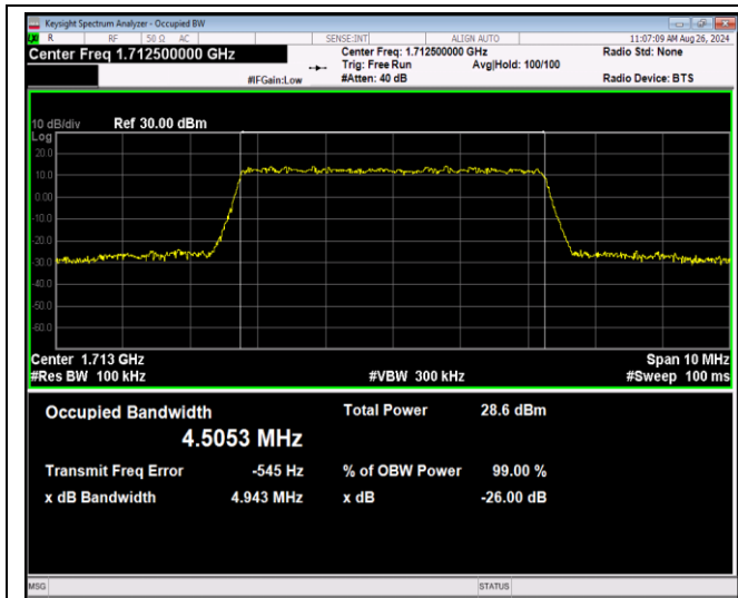
Band4-5MHz-QPSK-20375-25RB#0
