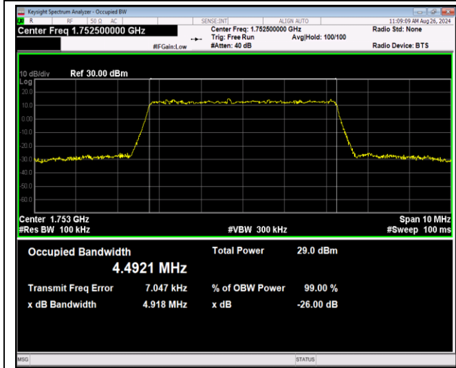
Band4-5MHz-16QAM-20175-25RB#0
