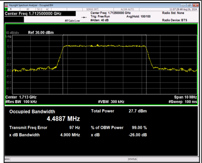
Band4-5MHz-16QAM-20375-25RB#0
