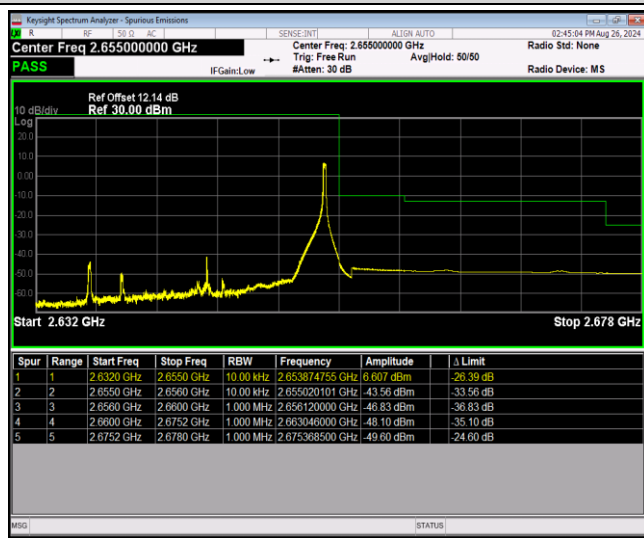
Band41-20MHz-64QAM-41140-1RB#99
