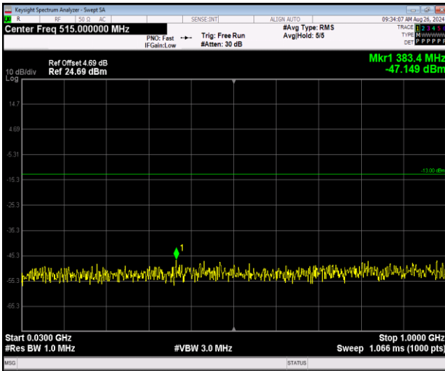
Band2-1.4MHz-64QAM-18607-1RB#0-Range1:30~10 00MHz
