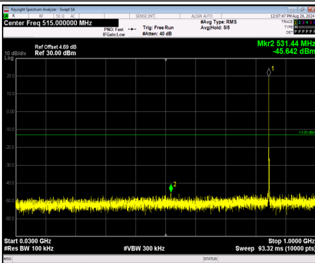
Band5-1.4MHz-64QAM-20407-1RB#0-Range1:30~10 00MHz
