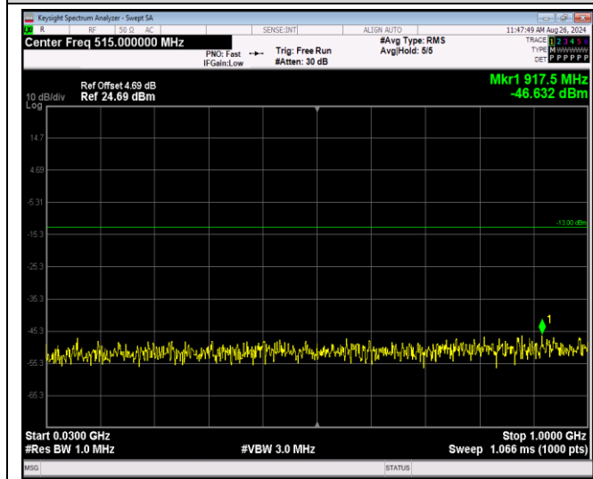
Band4-20MHz-64QAM-20175-1RB#0-Range1:30~100 OMHz
