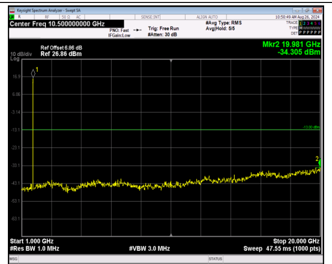
Band4-1.4MHz-16QAM-20393-1RB#0-Range2:1000~20000MHz
