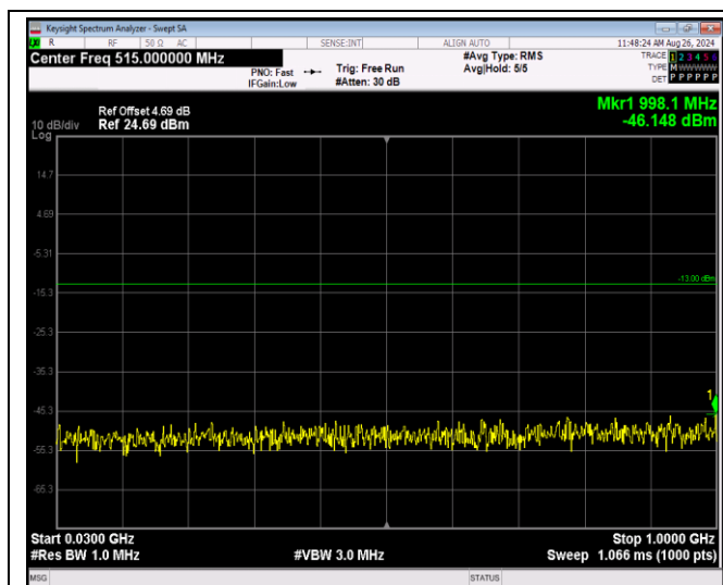
Band4-20MHz-64QAM-20050-1RB#0-Range1:30~100 OMHz
