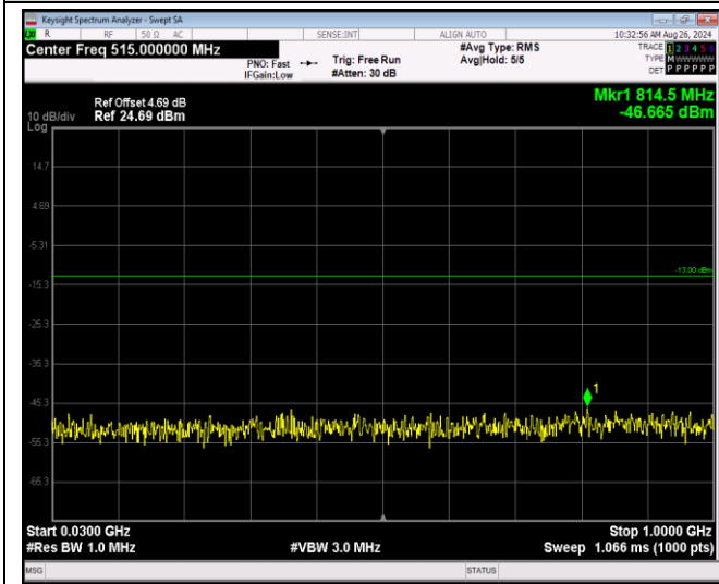
Band2-20MHz-16QAM-19100-1RB#0-Range1:30~100 0MHz
