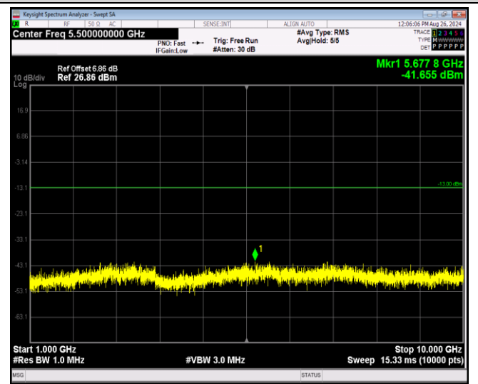
Band5-1.4MHz-16QAM-20407-1RB#0-Range2:1000~1 0000MHz
