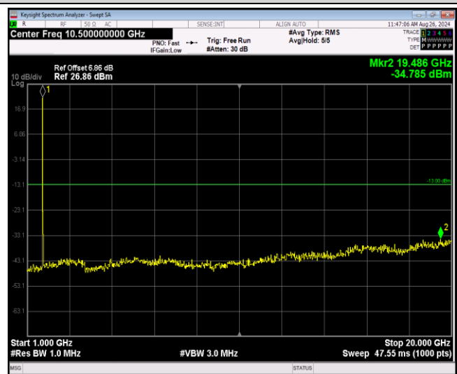
Band4-20MHz-64QAM-20175-1RB#0-Range2:1000~2 0000MHz
