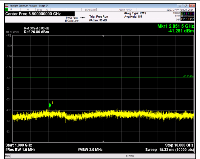
Band5-1.4MHz-16QAM-20407-1RB#0-Range2:1000~1 0000MHz
