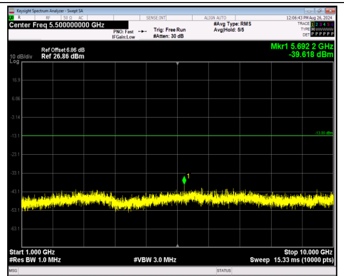
Band5-1.4MHz-QPSK-20643-1RB#0-Range2:1000~10 000MHz
