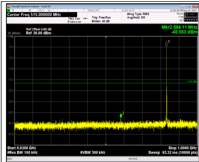
Band5-1.4MHz-QPSK-20643-1RB#0-Range1:30~100 OMHz
