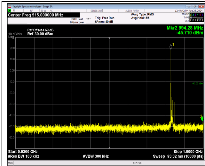
Band5-10MHz-64QAM-20600-1RB#0-Range1:30~100 OMHz
