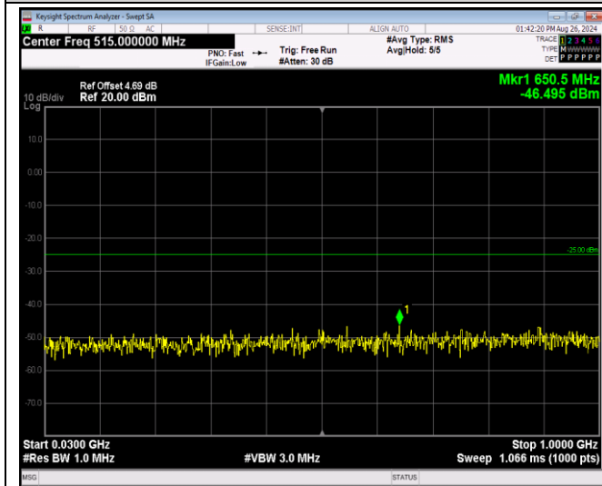
Band7-20MHz-64QAM-20850-1RB#0-Range1:30~100 OMHz
