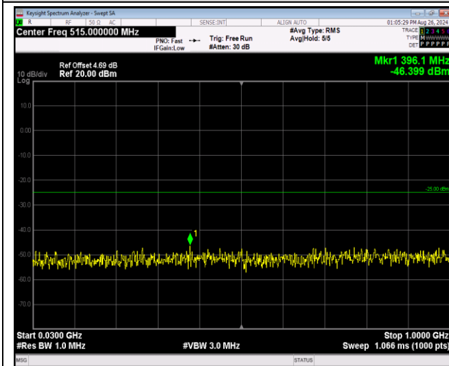
Band7-5MHz-16QAM-21425-1RB#0-Range1:30~1000 MHz
