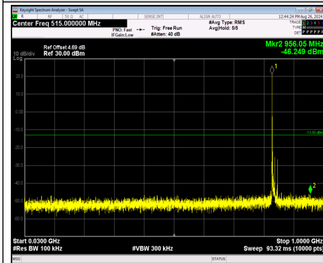
Band5-10MHz-16QAM-20525-1RB#0-Range1:30~100 OMHz
