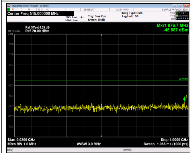
Band41-5MHz-QPSK-41215-1RB#0-Range1:30~1000 MHz
