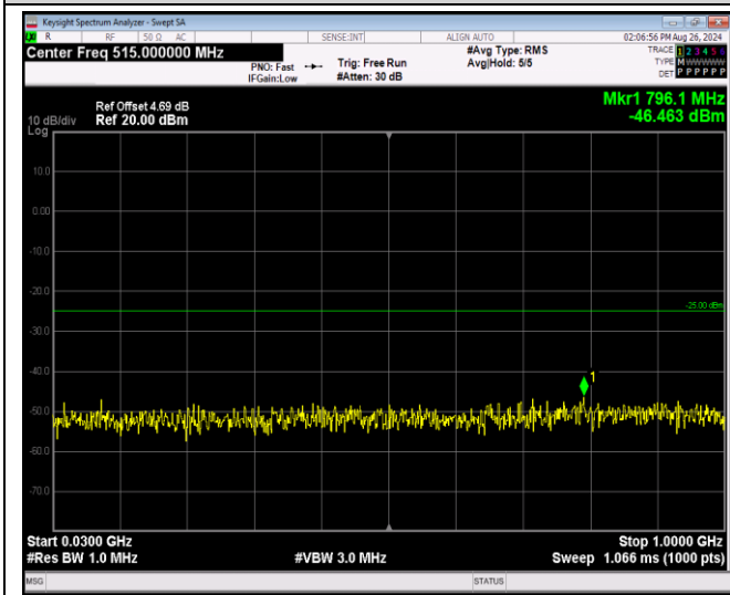
Band41-5MHz-64QAM-40640-1RB#0-Range1:30~100 OMHz
