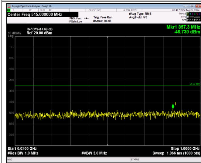
Band7-20MHz-64QAM-20850-1RB#0-Range1:30~100 OMHz
