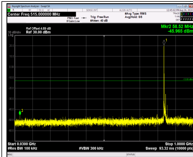
Band5-10MHz-16QAM-20450-1RB#0-Range1:30~100 OMHz
