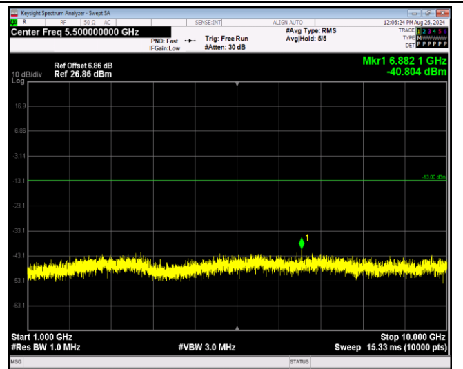
Band5-1.4MHz-64QAM-20525-1RB#0-Range2:1000~10000MHz
