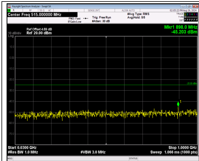
Band41-5MHz-QPSK-40640-1RB#0-Range1:30~1000 MHz
