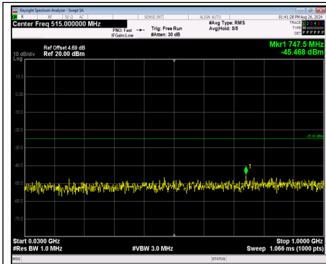
Band7-20MHz-16QAM-21350-1RB#0-Range1:30~100 OMHz
