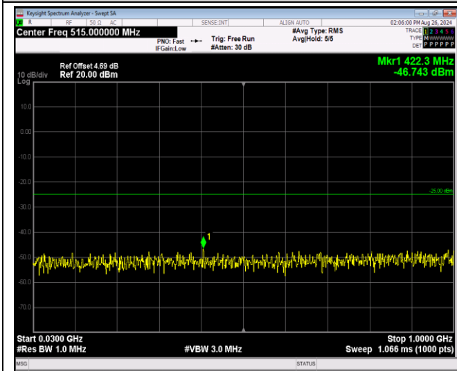
Band41-5MHz-64QAM-40640-1RB#0-Range1:30~100 OMHz
