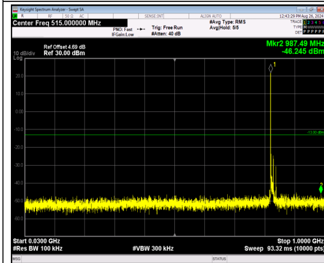
Band5-10MHz-16QAM-20525-1RB#0-Range1:30~100 OMHz
