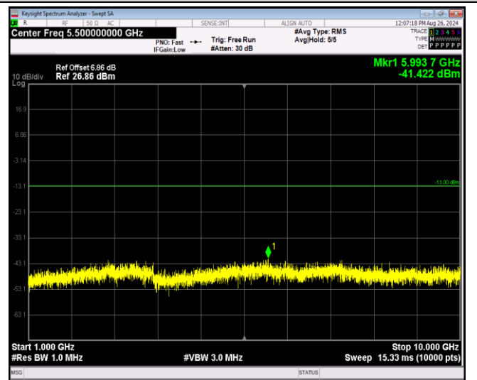
Band5-1.4MHz-64QAM-20643-1RB#0-Range2:1000~10000MHz
