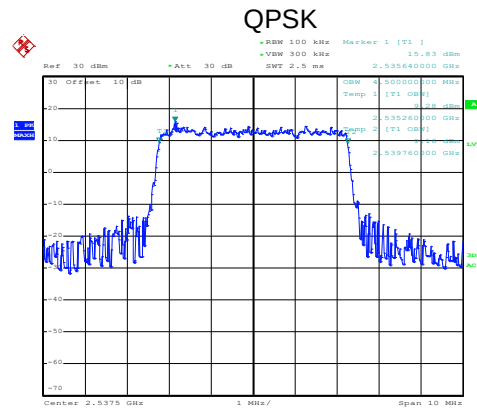
LTE Band 41: 99% Occupy bandwidth BW: 5MHz
