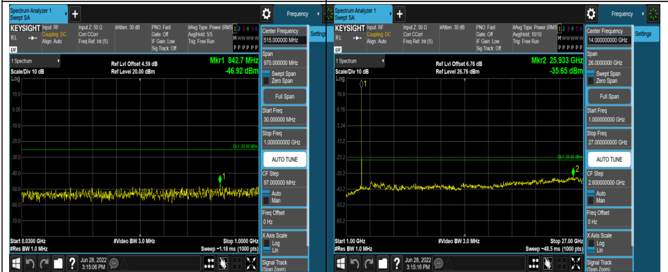
Band41-20MHz-16QAM-39750-1RB#0-Range1:30~1000MHz
