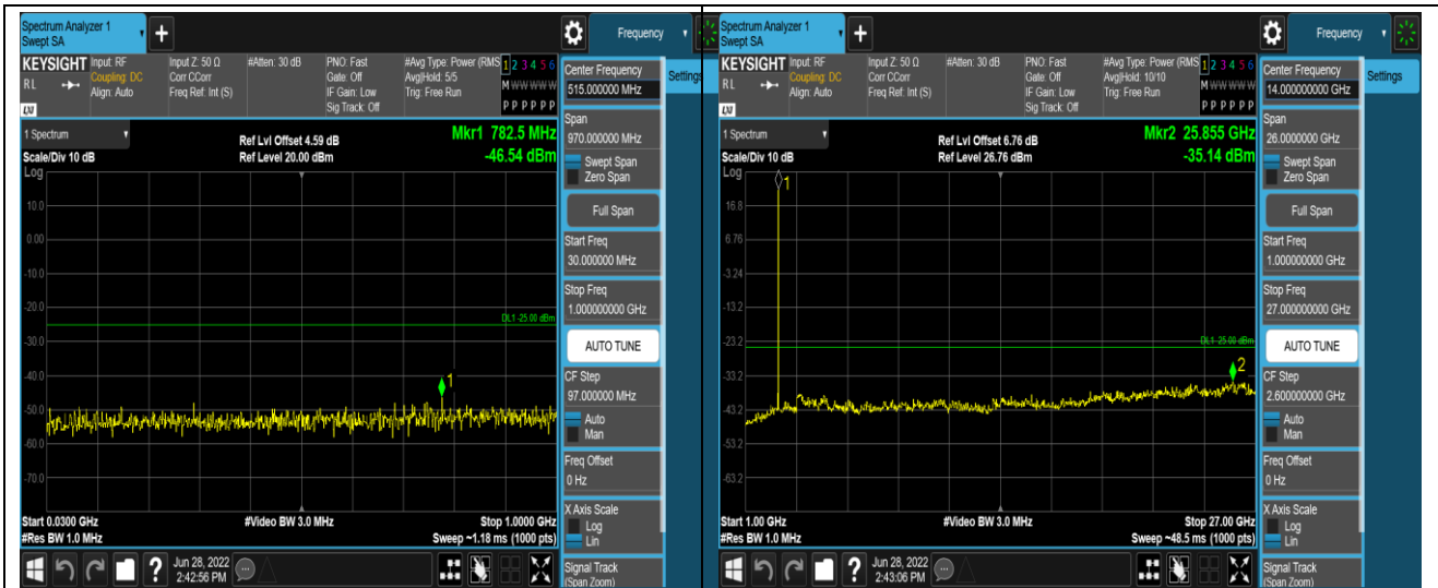
Band41-5MHz-16QAM-39675-1RB#0-Range1:30~1000MHz
