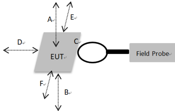
Figure 2: 20cm test setup
