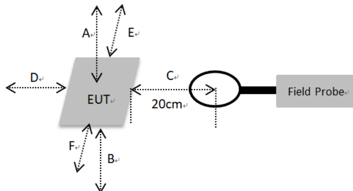
Figure 2: 20cm test setup
