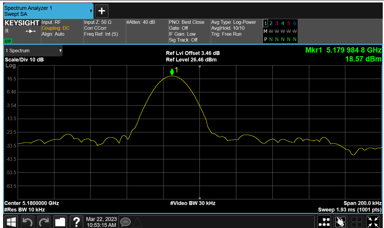
Freq. Stability NVHT a 5180MHz Ant6
