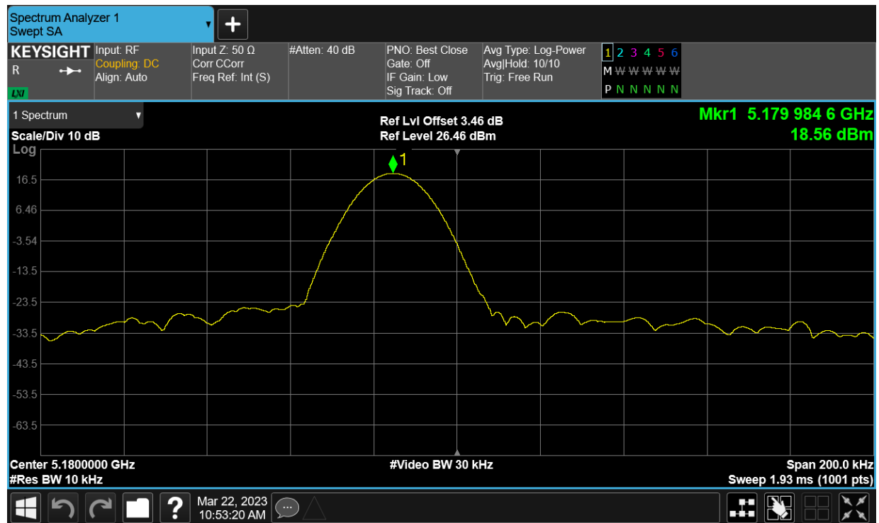
Freq. Stability LVNT a 5180MHz Ant6
