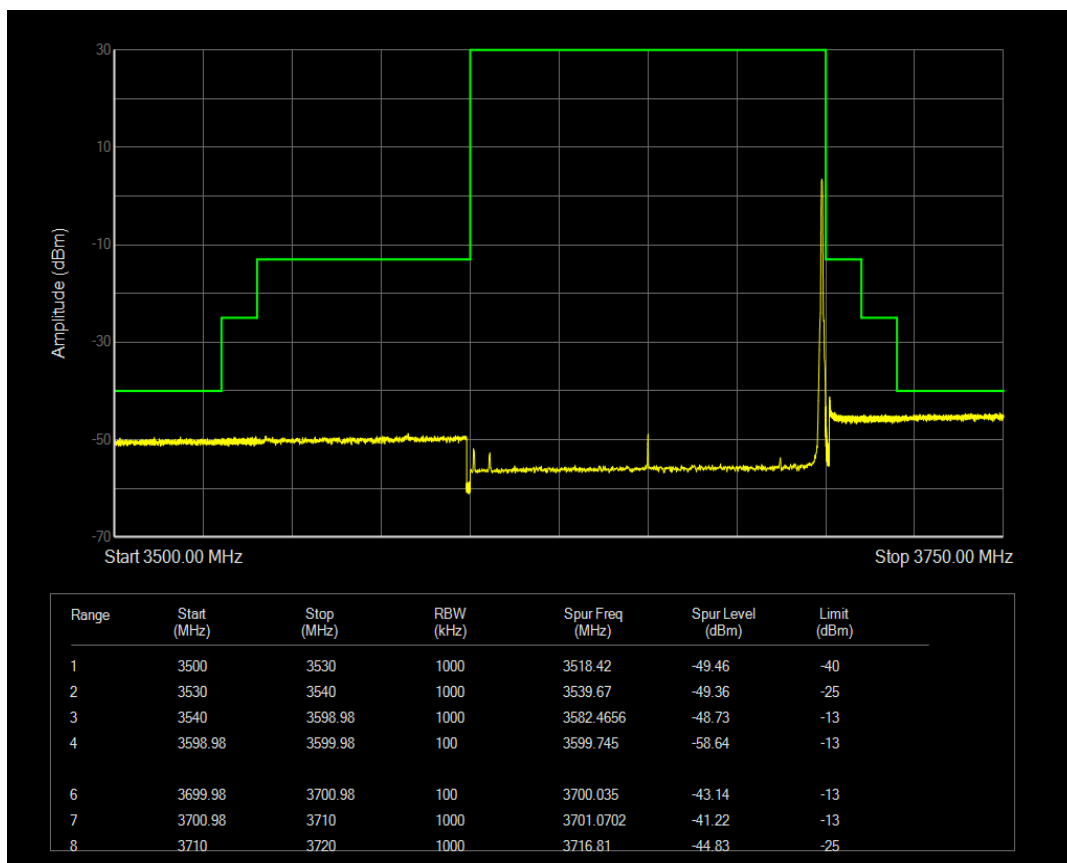
n78(3550-3700) SCS=30kHz CP_QPSK BW=100MHz Channel=643332 RB=273@0
