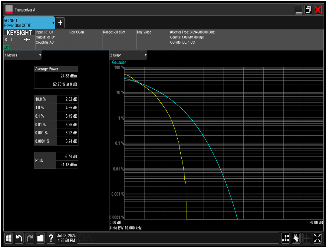
n77(3550-3700) SCS=30kHz DFT_QPSK BW=15MHz Channel=637168 RB=36@0
