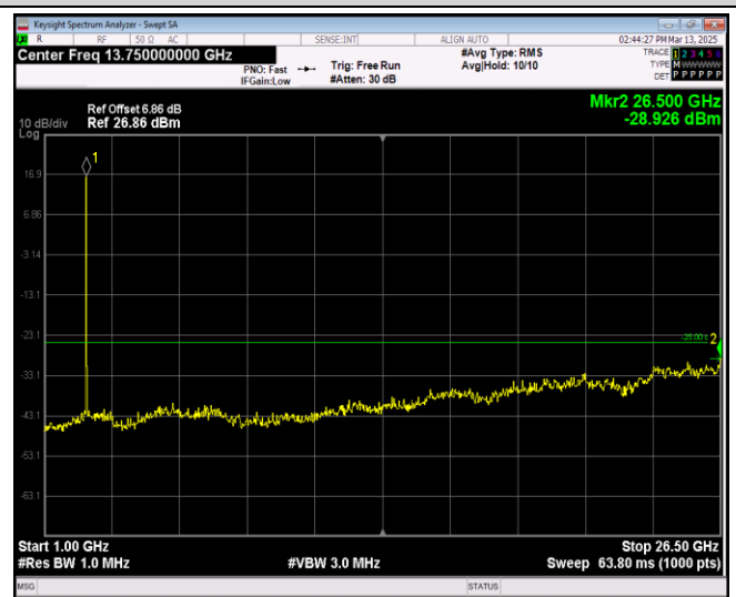
Band38-5MHz-64QAM-38000-1RB#0-Range2:1000~26500MHz
