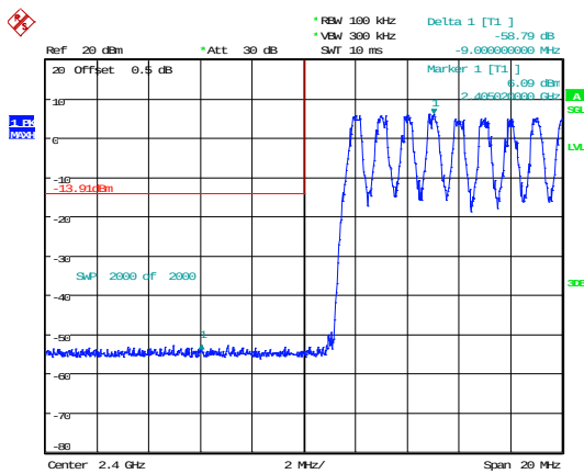
DH1_Hopping_Lower
