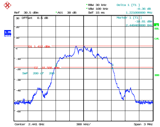
3DH1_Middle
