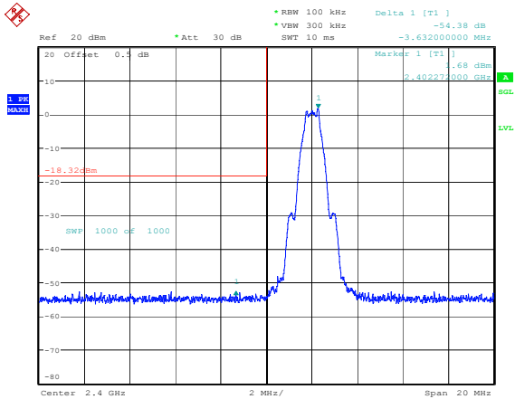
BLE_1M_Low_Channel
