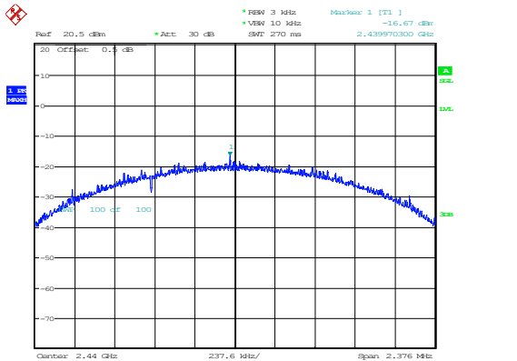
BLE_2M_Middle_Channel
