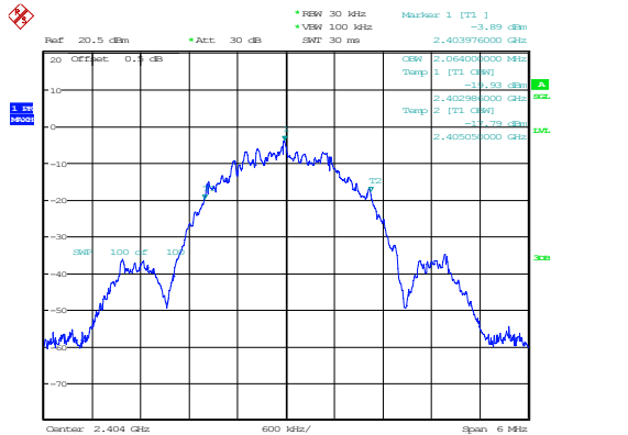
BLE_2M_Low_Channel
