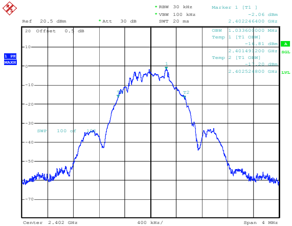
BLE_1M_Low_Channel
