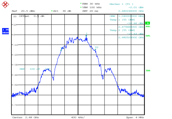
BLE_1M_High_Channel
