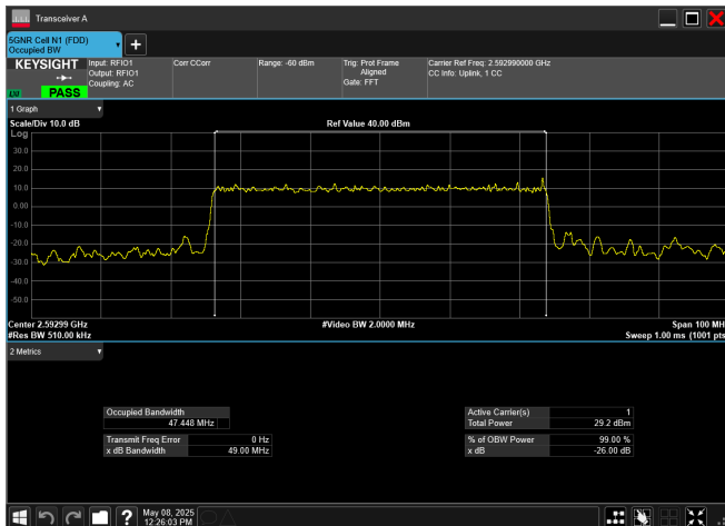
n41_50MHz_30kHz_2592.99MHz_CP-OFDM 64 QAM_RB133@0
