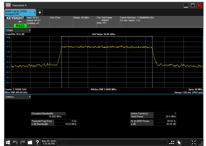
n66_20MHz_15kHz_1745MHz_CP-OFDM 256 QAM_RB106@0
