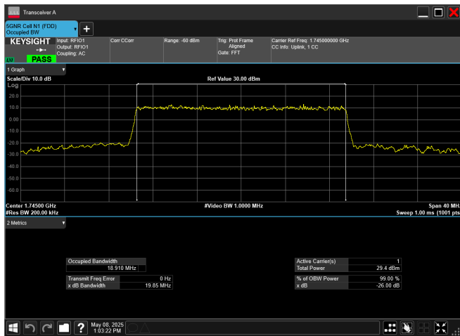
n66_20MHz_15kHz_1745MHz_CP-OFDM 64 QAM_RB106@0
