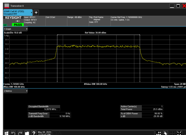
n66_10MHz_15kHz_1745MHz_CP-OFDM 256 QAM_RB52@0
