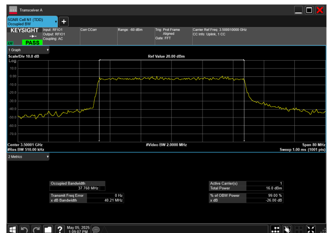
n77_1_40MHz_30kHz_3500MHz_CP-OFDM 256 QAM_RB106@0
