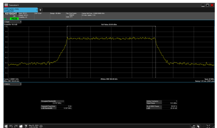
n77_1_10MHz_30kHz_3500MHz_CP-OFDM 256 QAM_RB24@0
