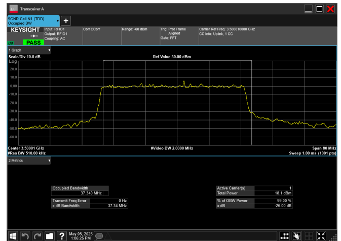
n77_1_40MHz_30kHz_3500MHz_CP-OFDM 16 QAM_RB106@0
