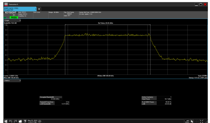
n77_1_10MHz_30kHz_3500MHz_CP-OFDM 16 QAM_RB24@0
