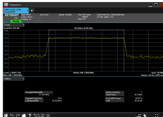
n77_1_60MHz_30kHz_3500MHz_CP-OFDM 16 QAM_RB162@0
