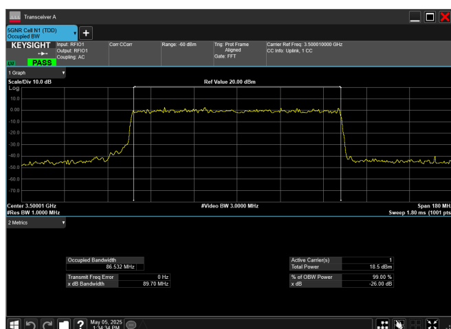
n77_1_90MHz_30kHz_3500MHz_DFT-s-OFDM 256 QAM_RB243@0
