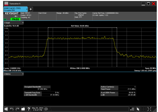
n77_3_40MHz_30kHz_3840MHz_DFT-s-OFDM 64 QAM_RB100@0
