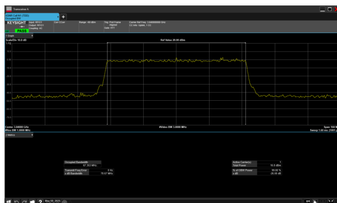
n77_3_70MHz_30kHz_3840MHz_CP-OFDM 256 QAM_RB189@0
