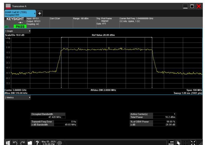
n77_3_50MHz_30kHz_3840MHz_CP-OFDM 256 QAM_RB133@0
