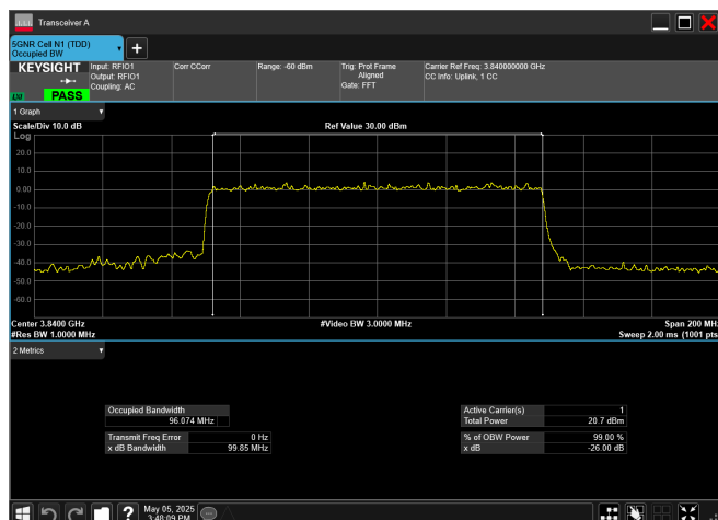
n77_3_100MHz_30kHz_3840MHz_DFT-s-OFDM 256 QAM_RB270@0
