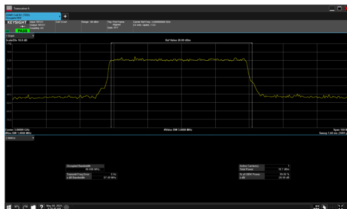
n77_3_70MHz_30kHz_3840MHz_CP-OFDM 16 QAM_RB189@0
