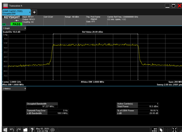
n77_3_100MHz_30kHz_3840MHz_CP-OFDM 256 QAM_RB273@0
