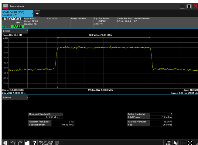
n77_3_90MHz_30kHz_3840MHz_CP-OFDM 64 QAM_RB245@0
