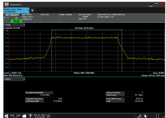
n78_1_15MHz_30kHz_3500MHz_DFT-s-OFDM 64 QAM_RB36@0
