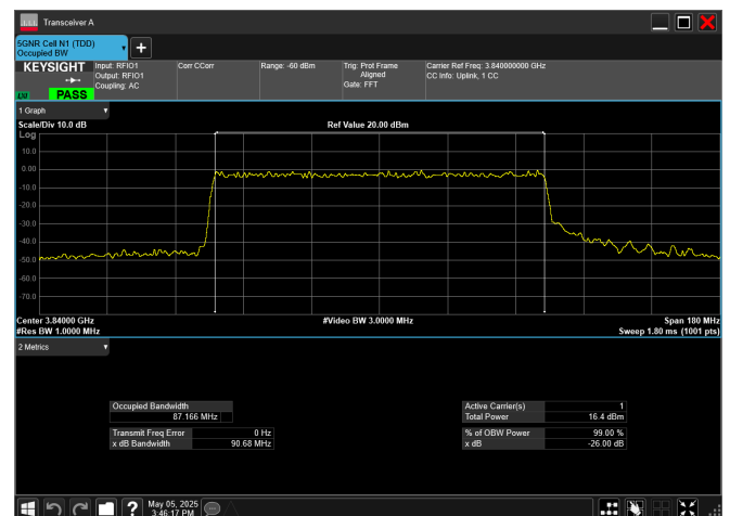
n77_3_90MHz_30kHz_3840MHz_CP-OFDM 256 QAM_RB245@0
