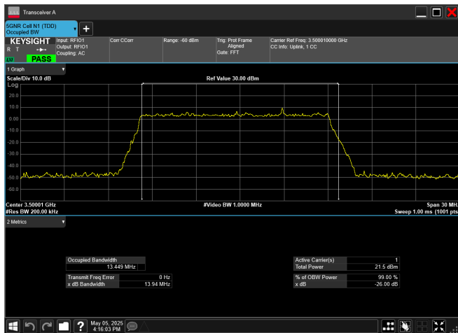
n78_1_15MHz_30kHz_3500MHz_DFT-s-OFDM 16 QAM_RB36@0
