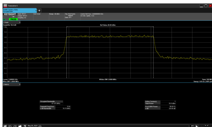
n77_3_70MHz_30kHz_3840MHz_CP-OFDM 64 QAM_RB189@0
