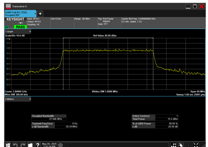
n77_3_30MHz_30kHz_3840MHz_CP-OFDM 256 QAM_RB78@0
