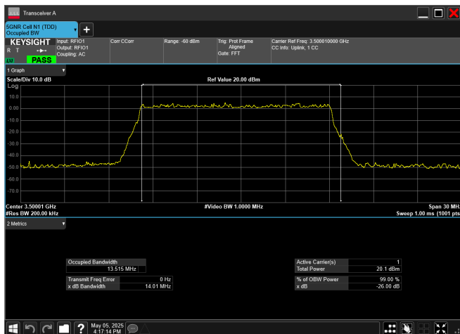
n78_1_15MHz_30kHz_3500MHz_DFT-s-OFDM 256 QAM_RB36@0
