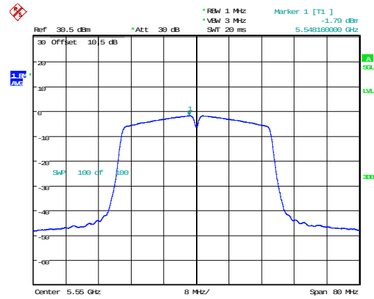
802.11n40_5550MHz
