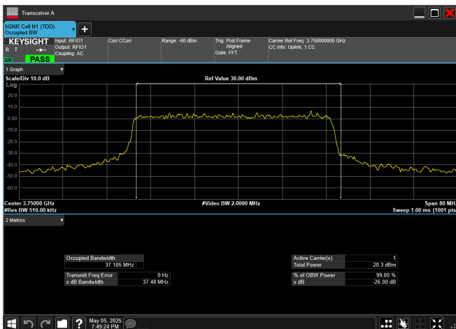
n78_3_40MHz_30kHz_3750MHz_DFT-s-OFDM 256 QAM_RB100@0
