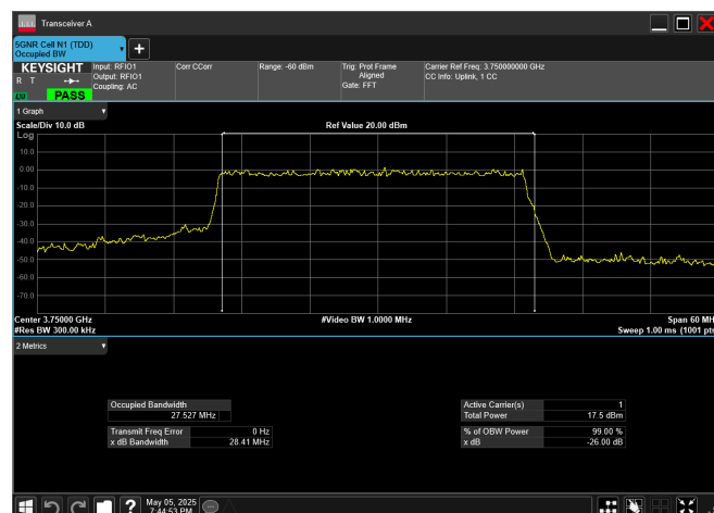
n78_3_30MHz_30kHz_3750MHz_CP-OFDM 16 QAM_RB78@0
