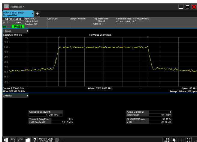
n78_3_50MHz_30kHz_3750MHz_CP-OFDM 64 QAM_RB133@0
