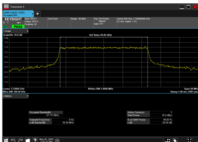
n78_3_30MHz_30kHz_3750MHz_CP-OFDM 64 QAM_RB78@0
