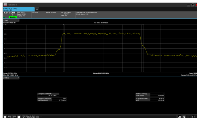
n78_3_70MHz_30kHz_3750MHz_CP-OFDM 16 QAM_RB189@0
