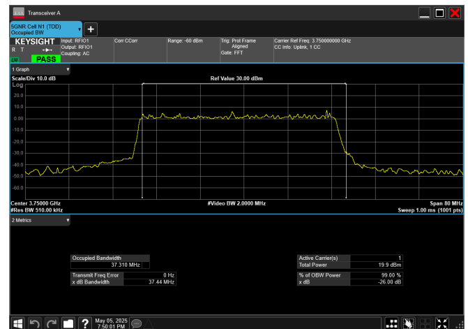
n78_3_40MHz_30kHz_3750MHz_DFT-s-OFDM 64 QAM_RB100@0
