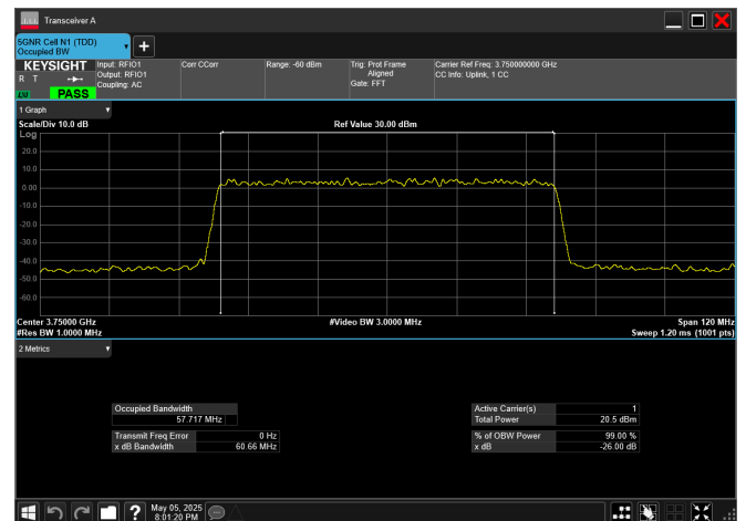
n78_3_60MHz_30kHz_3750MHz_DFT-s-OFDM 64 QAM_RB162@0
