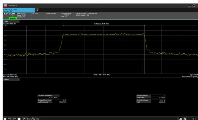
n78_3_70MHz_30kHz_3750MHz_CP-OFDM 256 QAM_RB189@0
