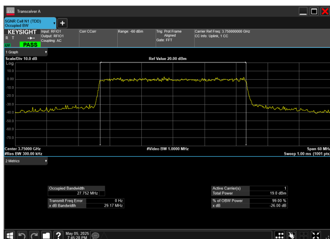
n78_3_30MHz_30kHz_3750MHz_CP-OFDM 64 QAM_RB78@0
