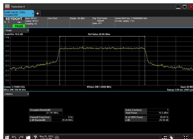
n78_3_30MHz_30kHz_3750MHz_CP-OFDM 256 QAM_RB78@0
