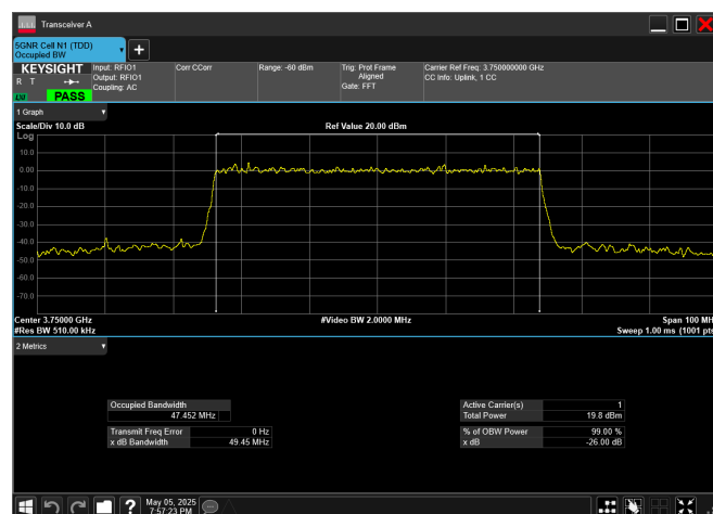
n78_3_50MHz_30kHz_3750MHz_CP-OFDM 256 QAM_RB133@0
