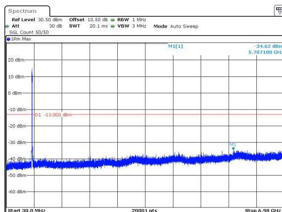
n71_15MHz_15kHz_670.5MHz_DFT-s-OFDM QPSK_RB75@0 -34.62dBm
