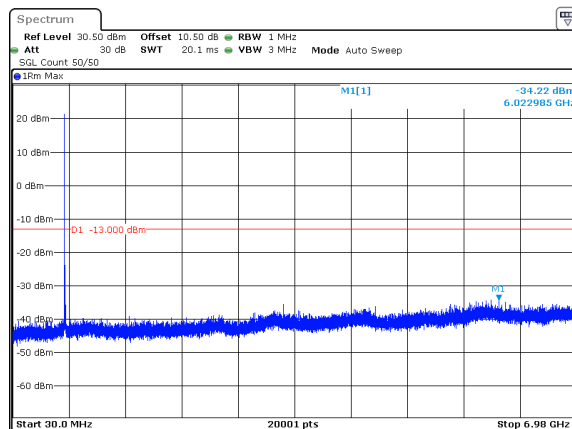
n71_15MHz_15kHz_670.5MHz_DFT-s-OFDM QPSK_RB1@0 -34.22dBm
