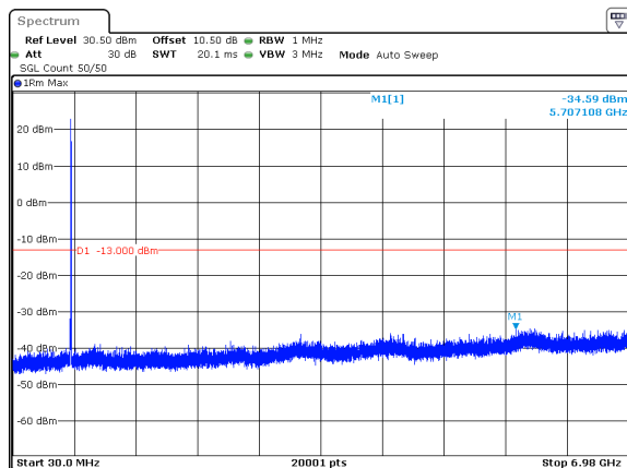
n71_10MHz_15kHz_680.5MHz_DFT-s-OFDM QPSK_RB1@51 -34.59dBm
