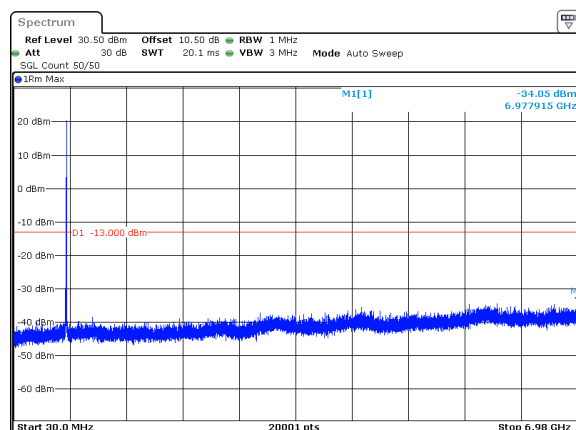
n71_15MHz_15kHz_670.5MHz_DFT-s-OFDM QPSK_RB1@78 -34.05dBm
