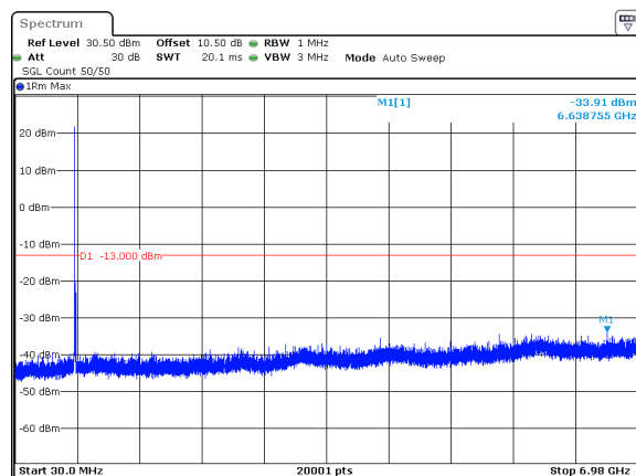
n71_10MHz_15kHz_693MHz_DFT-s-OFDM QPSK_RB1@0 -33.91dBm
