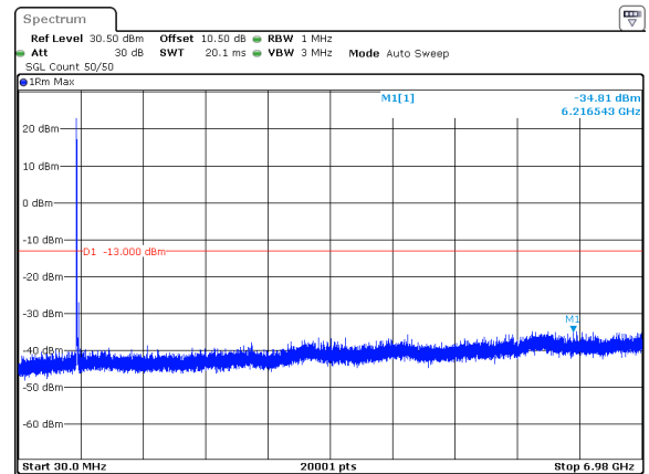
n71_10MHz_15kHz_680.5MHz_DFT-s-OFDM QPSK_RB1@0 -34.81dBm
