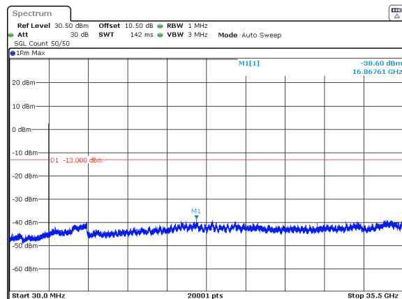
n77_1_15MHz_30kHz_3542.5MHz_DFT-s-OFDM QPSK_RB36@0 -38.60dBm
