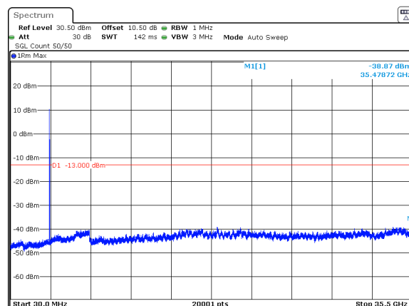
n77_1_15MHz_30kHz_3457.5MHz_DFT-s-OFDM QPSK_RB1@37 -38.87dBm
