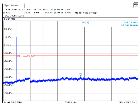
n77_1_15MHz_30kHz_3500MHz_DFT-s-OFDM QPSK_RB1@37 -39.03dBm
