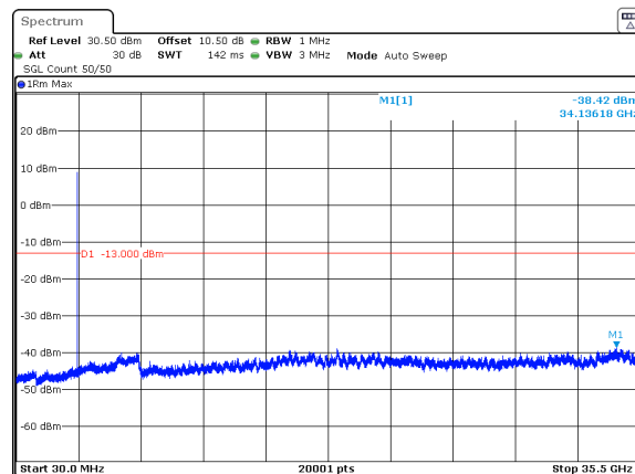
n77_1_15MHz_30kHz_3500MHz_DFT-s-OFDM QPSK_RB1@0 -38.42dBm
