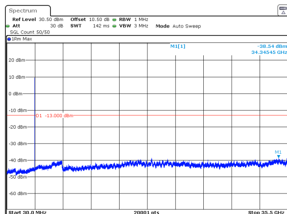
n77_1_15MHz_30kHz_3542.5MHz_DFT-s-OFDM QPSK_RB1@0 -38.54dBm
