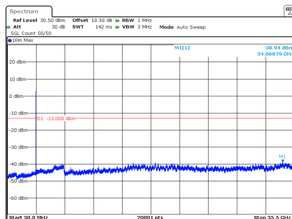
n77_1_15MHz_30kHz_3500MHz_DFT-s-OFDM QPSK_RB36@0 -38.94dBm
