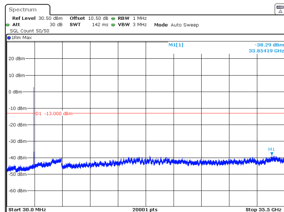
n77_1_15MHz_30kHz_3457.5MHz_DFT-s-OFDM QPSK_RB36@0 -38.29dBm
