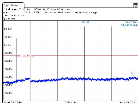
n77_1_15MHz_30kHz_3457.5MHz_DFT-s-OFDM QPSK_RB1@0 -38.47dBm
