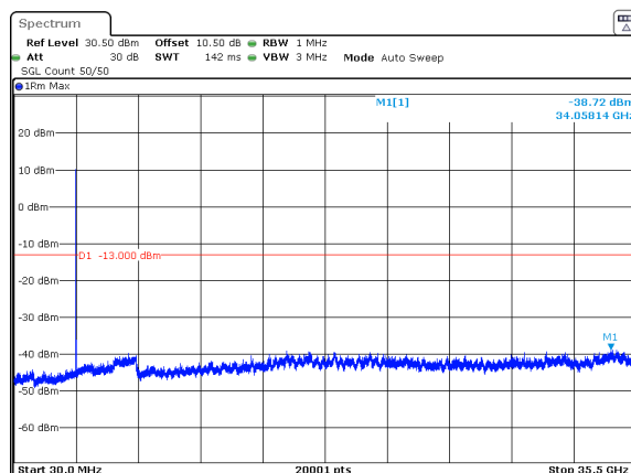
n77_1_15MHz_30kHz_3542.5MHz_DFT-s-OFDM QPSK_RB1@37 -38.72dBm
