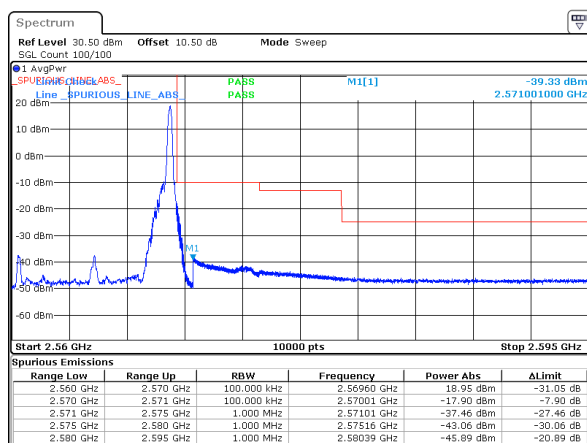
n7_10MHz_15kHz_2565MHz_DFT-s-OFDM QPSK_RB1@51
