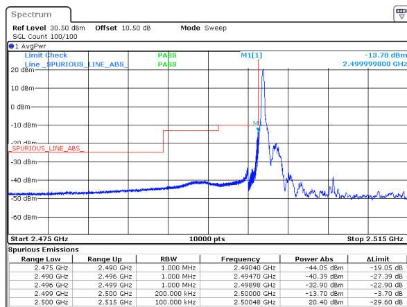
n7_15MHz_15kHz_2507.5MHz_DFT-s-OFDM QPSK_RB1@0
