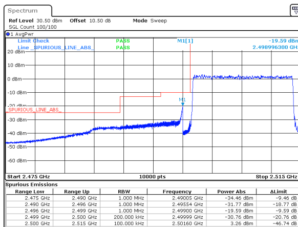
n7_15MHz_15kHz_2507.5MHz_DFT-s-OFDM QPSK_RB75@0
