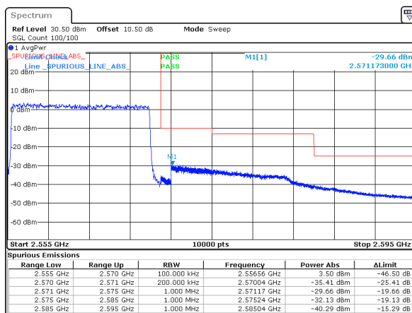
n7_15MHz_15kHz_2562.5MHz_DFT-s-OFDM QPSK_RB75@0
