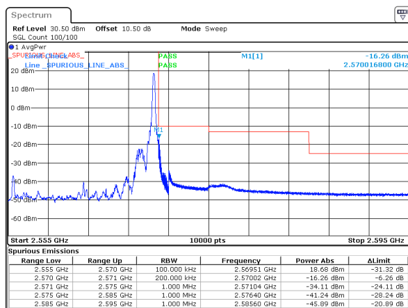
n7_15MHz_15kHz_2562.5MHz_DFT-s-OFDM QPSK_RB1@78
