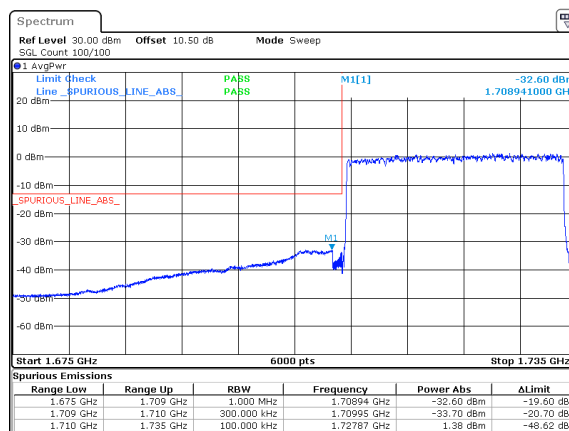
n66_25MHz_15kHz_1722.5MHz_DFT-s-OFDM QPSK_RB128@0
