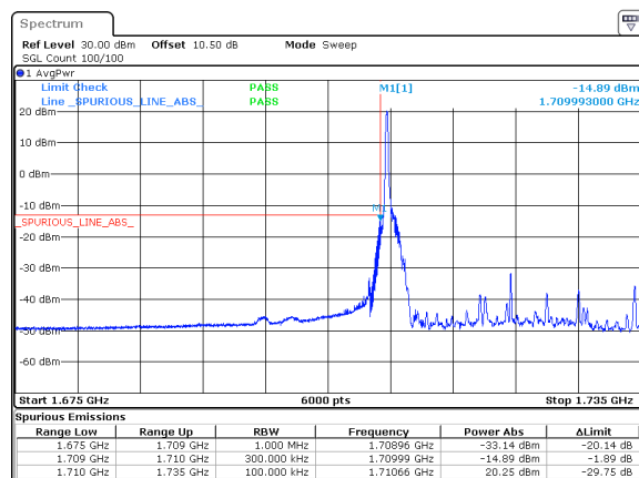
n66_25MHz_15kHz_1722.5MHz_DFT-s-OFDM QPSK_RB1@0
