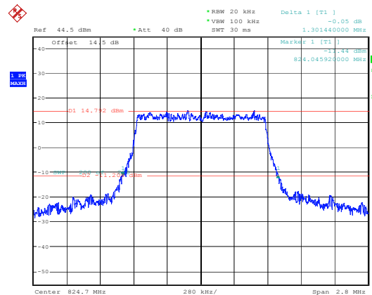
26dB Bandwidth
