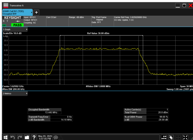
n78_2_15MHz_30kHz_3625MHz_DFT-s-OFDM 16 QAM_RB36@0
