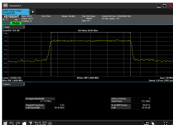
n78_2_60MHz_30kHz_3625MHz_CP-OFDM 64 QAM_RB162@0
