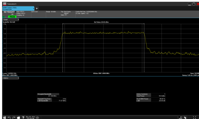
n78_2_70MHz_30kHz_3625MHz_CP-OFDM 256 QAM_RB189@0
