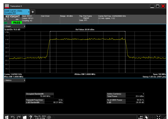
n78_2_80MHz_30kHz_3625MHz_DFT-s-OFDM 16 QAM_RB216@0
