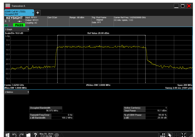
n78_2_100MHz_30kHz_3625MHz_CP-OFDM 256 QAM_RB273@0
