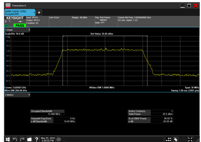
n78_2_15MHz_30kHz_3625MHz_DFT-s-OFDM 64 QAM_RB36@0
