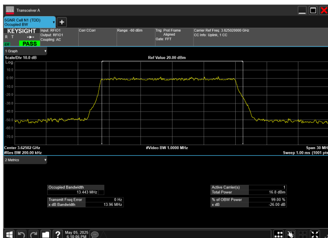
n78_2_15MHz_30kHz_3625MHz_DFT-s-OFDM 256 QAM_RB36@0
