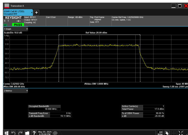
n78_2_20MHz_30kHz_3625MHz_CP-OFDM 16 QAM_RB51@0
