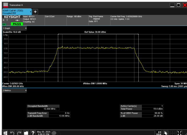
n78_2_15MHz_30kHz_3625MHz_DFT-s-OFDM 256 QAM_RB36@0
