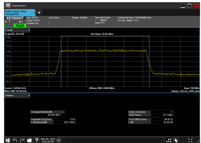
n78_2_50MHz_30kHz_3625MHz_DFT-s-OFDM 64 QAM_RB128@0
