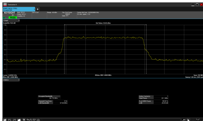
n78_2_70MHz_30kHz_3625MHz_DFT-s-OFDM 16 QAM_RB180@0
