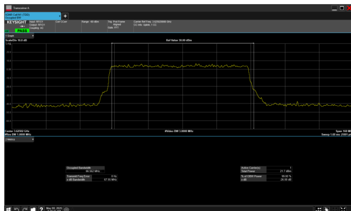
n78_2_70MHz_30kHz_3625MHz_DFT-s-OFDM 64 QAM_RB180@0
