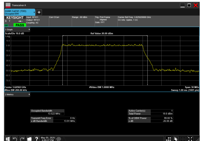
n78_2_15MHz_30kHz_3625MHz_DFT-s-OFDM 64 QAM_RB36@0
