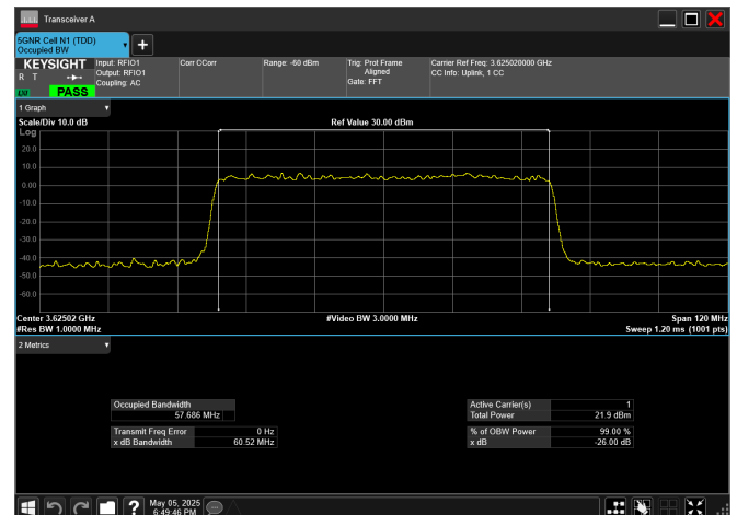
n78_2_60MHz_30kHz_3625MHz_DFT-s-OFDM 16 QAM_RB162@0
