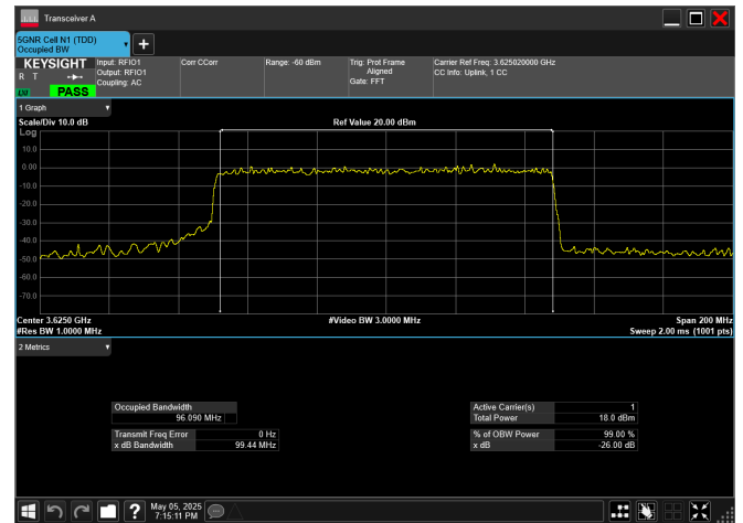
n78_2_100MHz_30kHz_3625MHz_CP-OFDM 16 QAM_RB273@0
