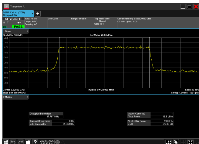
n78_2_40MHz_30kHz_3625MHz_CP-OFDM 64 QAM_RB106@0
