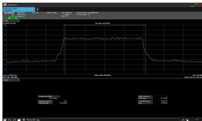
n78_2_70MHz_30kHz_3625MHz_DFT-s-OFDM 256 QAM_RB180@0
