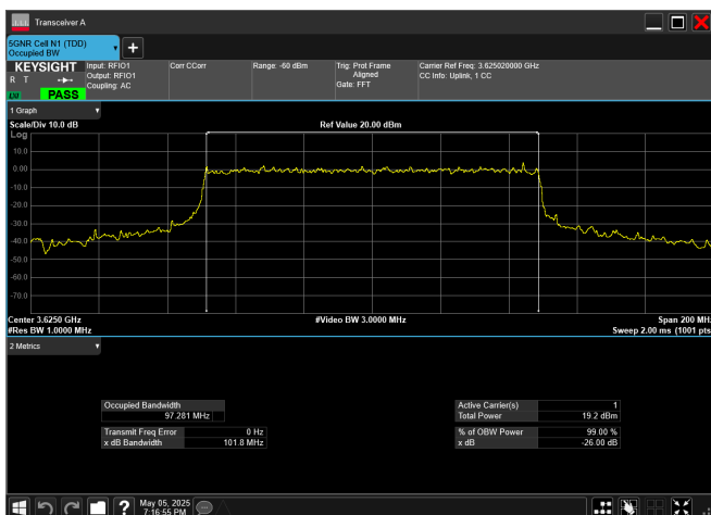
n78_2_100MHz_30kHz_3625MHz_CP-OFDM 64 QAM_RB273@0
