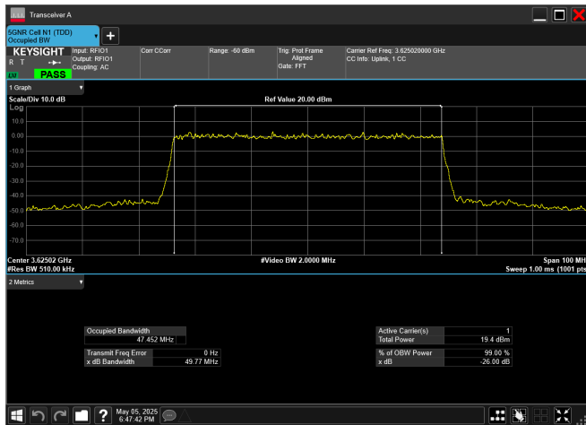
n78_2_50MHz_30kHz_3625MHz_CP-OFDM 256 QAM_RB133@0
