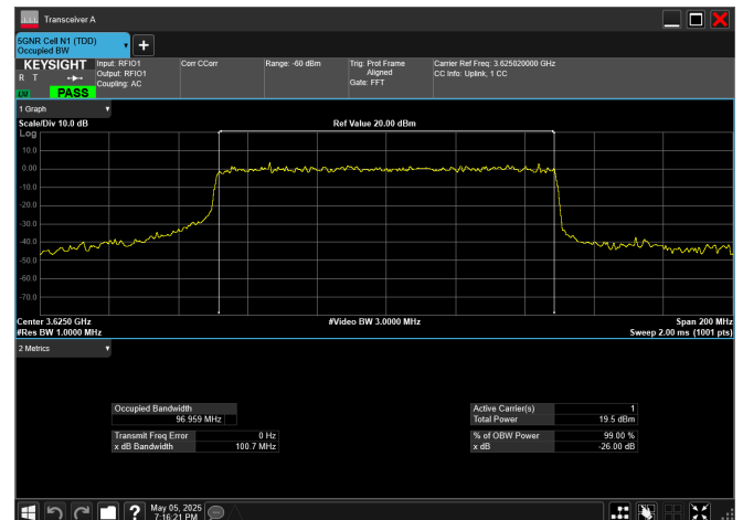
n78_2_100MHz_30kHz_3625MHz_CP-OFDM 256 QAM_RB273@0
