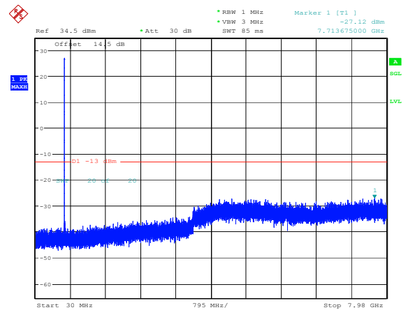
5MHz_Middle_QPSK_1@0(30MHz~7.98GHz)
