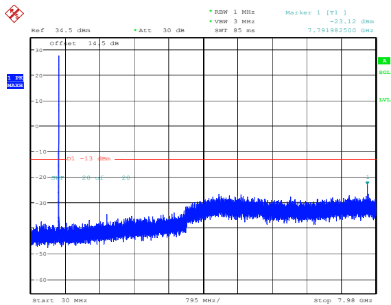
5MHz_Low_QPSK_1@0(30MHz~7.98GHz)
