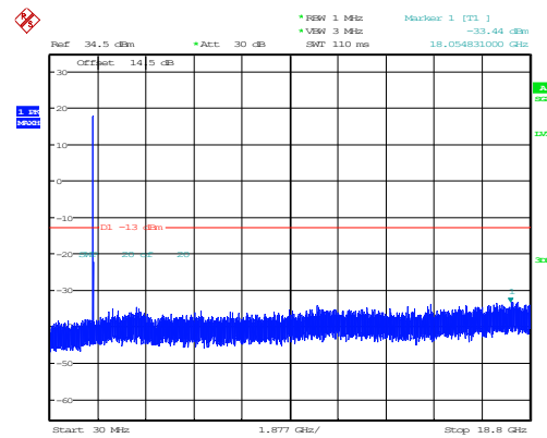
3MHz_Low_QPSK_1@0(30MHz~18.8GHz)
