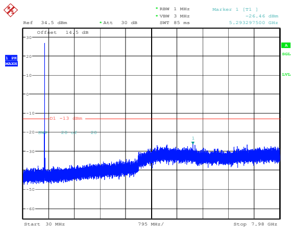
5MHz_High_QPSK_1@0(30MHz~7.98GHz)
