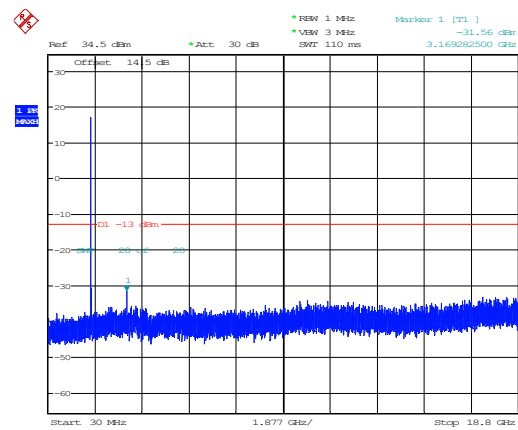
15MHz_Middle_QPSK_1@0(30MHz~18.8GHz)
