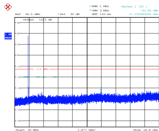
20MHz_High_QPSK_1@0(30MHz~18.8GHz)
