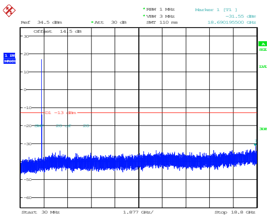
15MHz_Low_QPSK_1@0(30MHz~18.8GHz)
