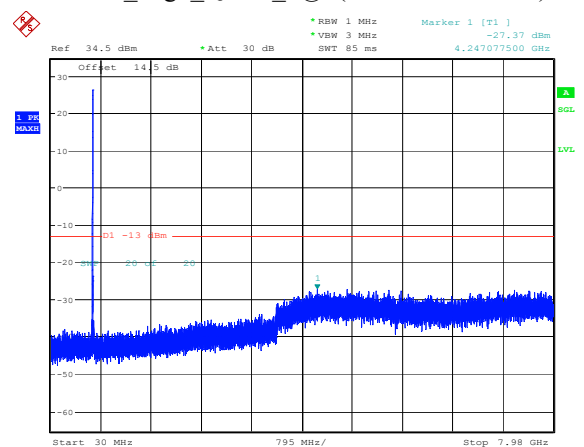
10MHz_High_QPSK_1@0(30MHz~7.98GHz)
