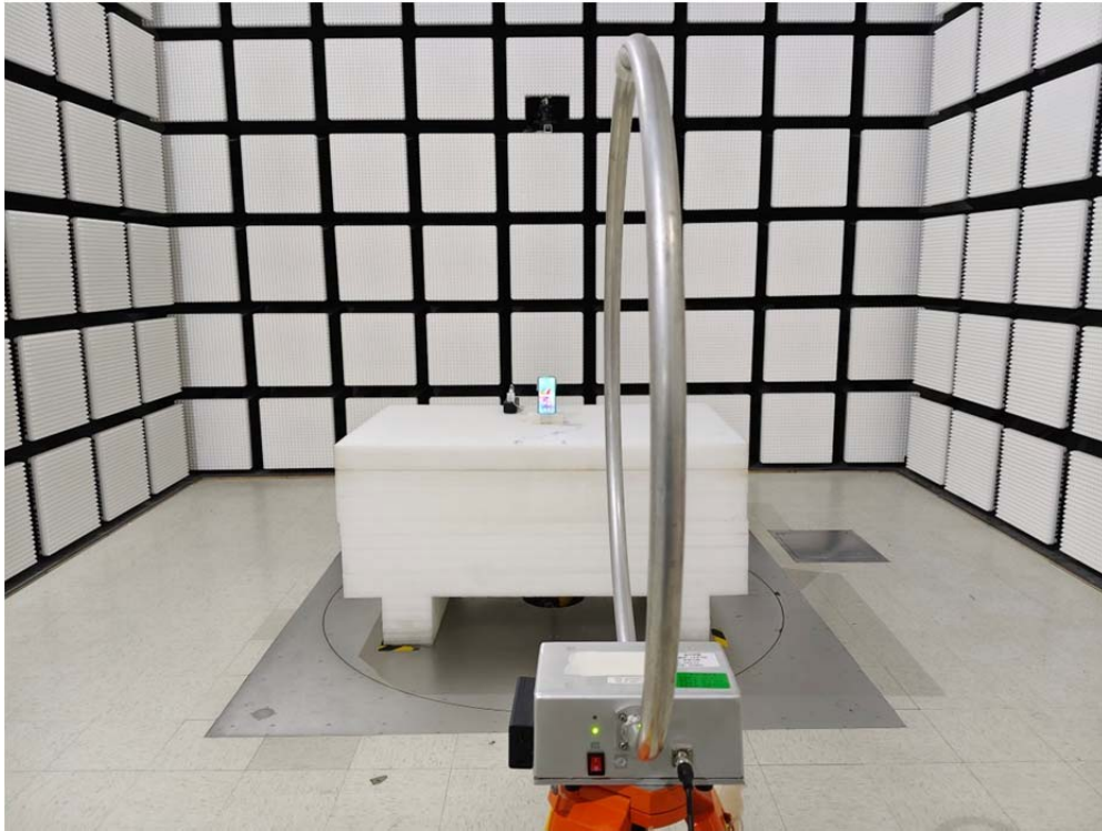
Radiated Emission 9 kHz-30 MHz Perpendicular View_Type 1
