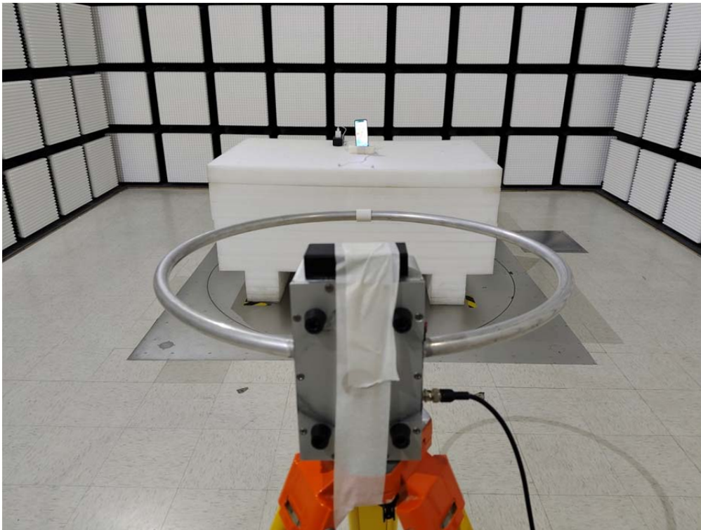
Radiated Emission 9 kHz-30 MHz Ground-parallel View_Type 1
