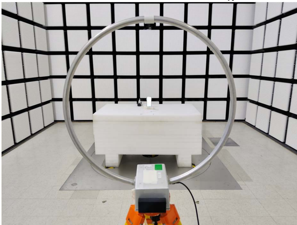
Radiated Emission 9 kHz-30 MHz Parallel View_Type 1
