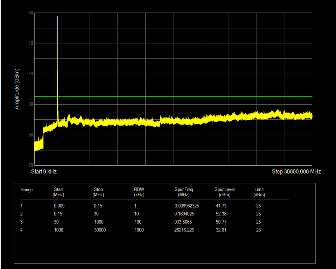
n41(2535-2655) SCS=15kHz DFT_QPSK BW=50MHz Channel=512004 RB=1@269
