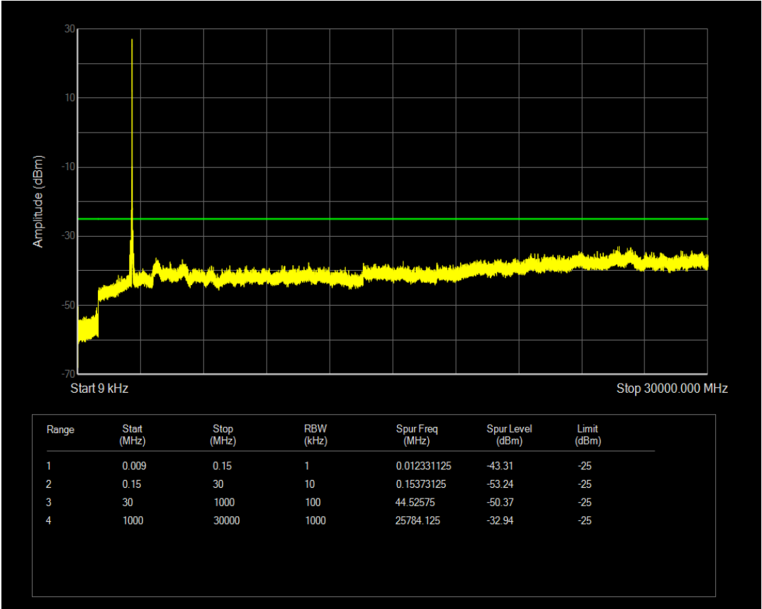
n41(2535-2655) SCS=15kHz DFT_QPSK BW=50MHz Channel=525996 RB=1@269
