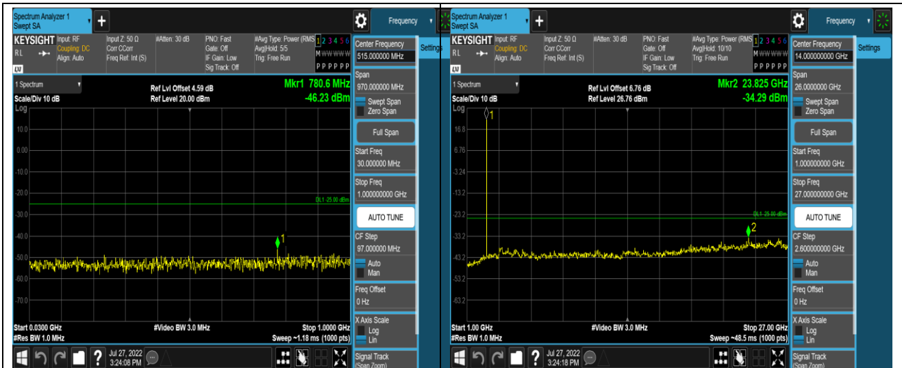
Band41-5MHz-QPSK-41565-1RB#0-Range1:30~1000MHz
