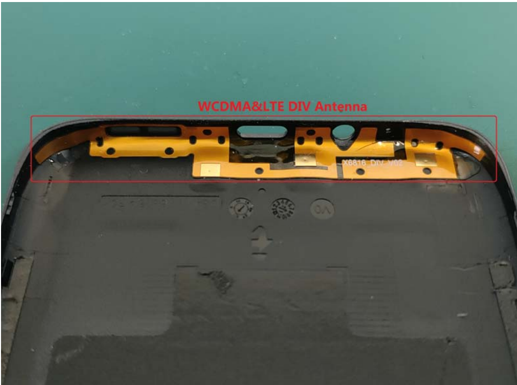
DIV Antenna
