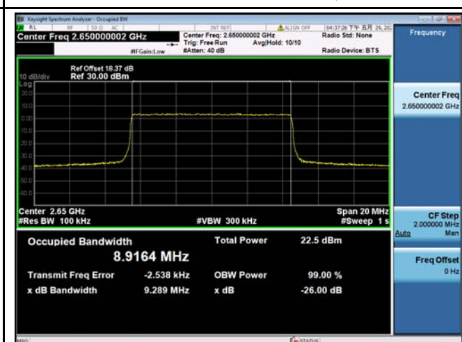
LTE band 41 - Middle CH 16QAM-10
