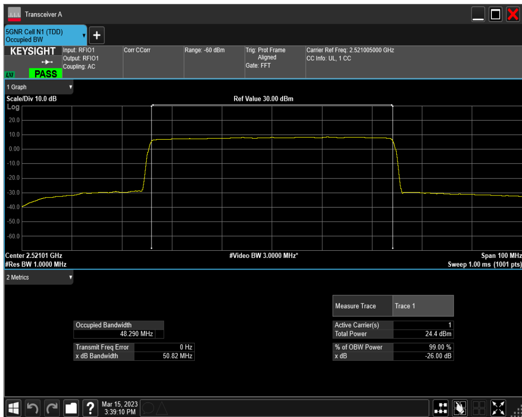
n41 SCS=15kHz DFT_QAM256 BW=50MHz Channel=504201 RB=270@0
