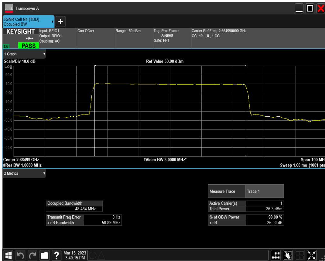
n41 SCS=15kHz DFT_QPSK BW=50MHz Channel=532998 RB=270@0
