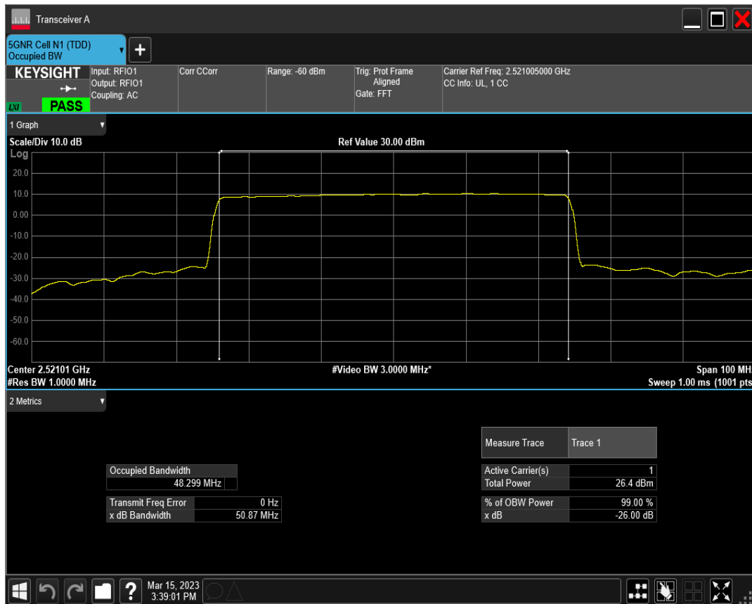
n41 SCS=15kHz DFT_QPSK BW=50MHz Channel=504201 RB=270@0
