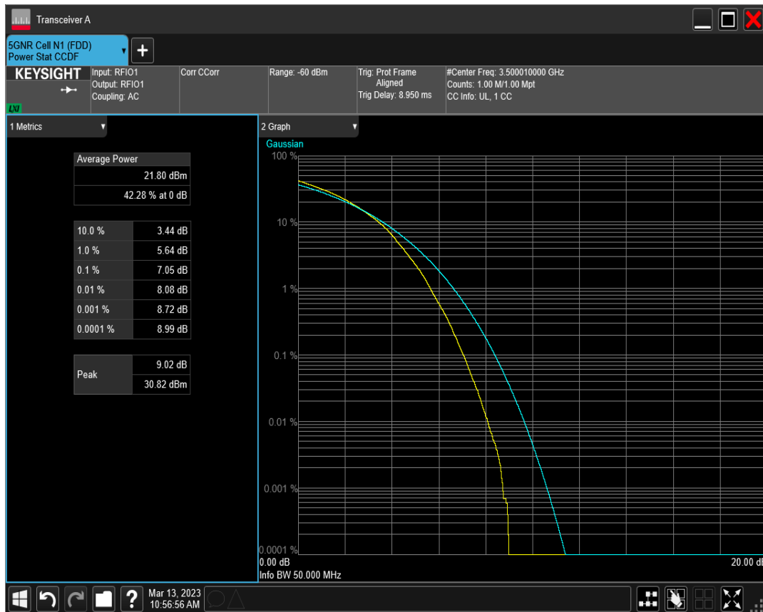
n77(3450-3550) SCS=15kHz DFT_BPSK BW=50MHz Channel=633334 RB=270@0
