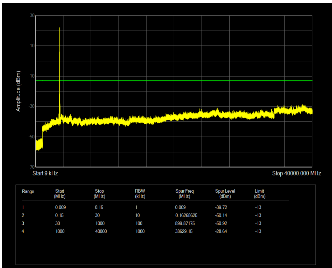
n77(3450-3550) SCS=30kHz DFT_QPSK BW=100MHz Channel=633334 RB=1@272
